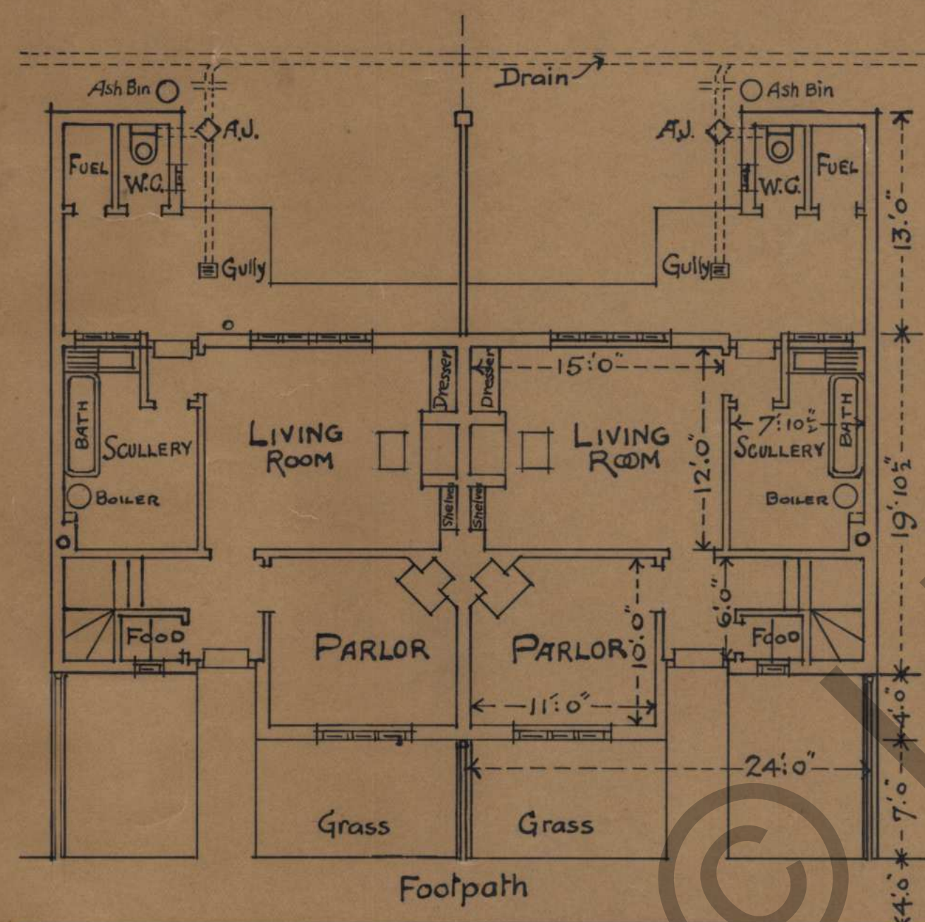
PLAN OF GROUND FLOOR
