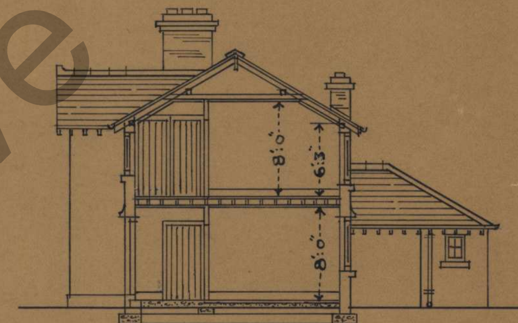
SECTION
