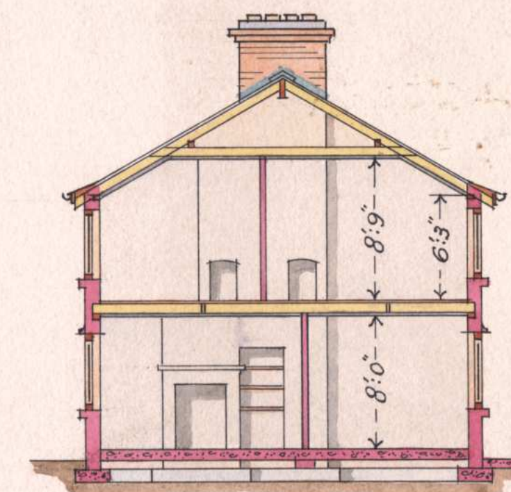
SECTION
