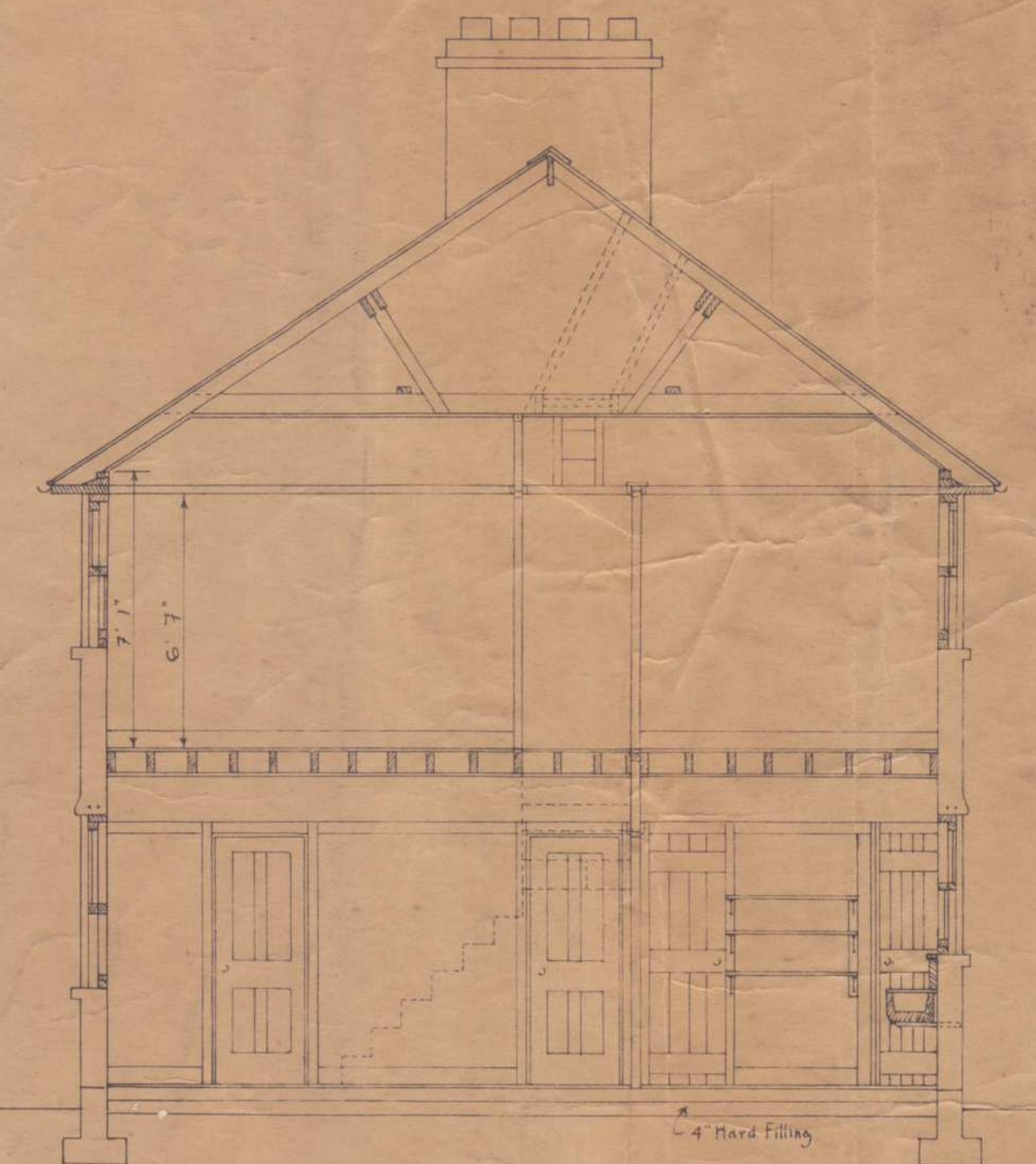
- SECTION -
