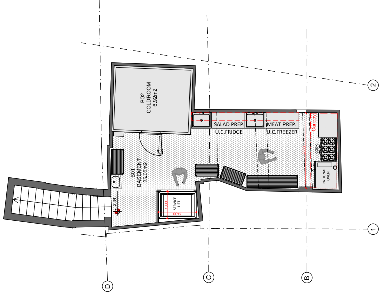
BASEMENT FLOOR ALTERNATIVE 2
