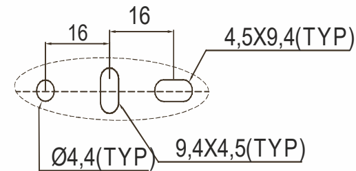
B Detail (2:1)
