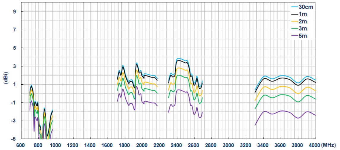
Peak Gain (dBi) - LTE MIMO1
