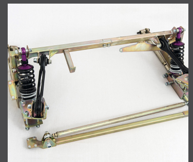
SSL Suspension
