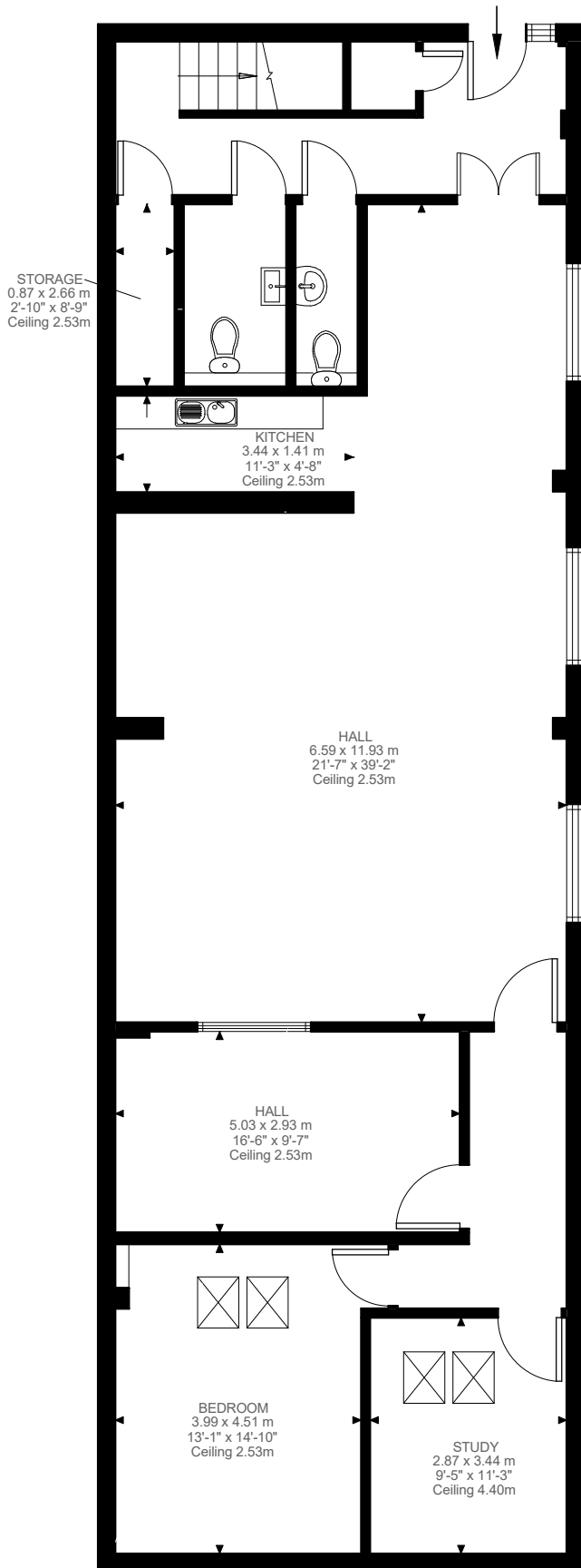
Ground Floor 1571 ft²
