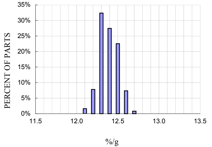
X-axis Sensitivity Distribution at Xout, V_{DD}=5V
