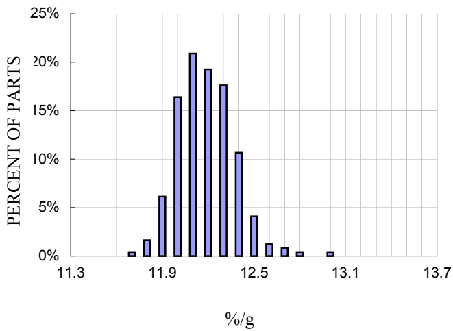
X-axis Sensitivity Distribution at Xout, V_{DD}=3V
