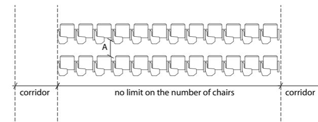
A ≥ 30cm in rows up to 14 chairs. 1,25cm for each additional chair up to 30 chairs max. A > 50cm: For 30 chairs or more. There is no limit on the number of chairs on each row, as long as the escape route until the door is equal or less than 25 metres.
