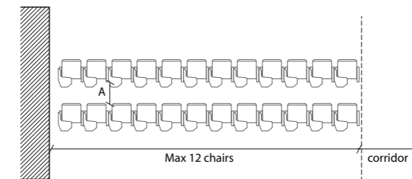
A ≥ 30cm for 7 chairs 2,5cm for each additional chair up to 12 chairs max.
