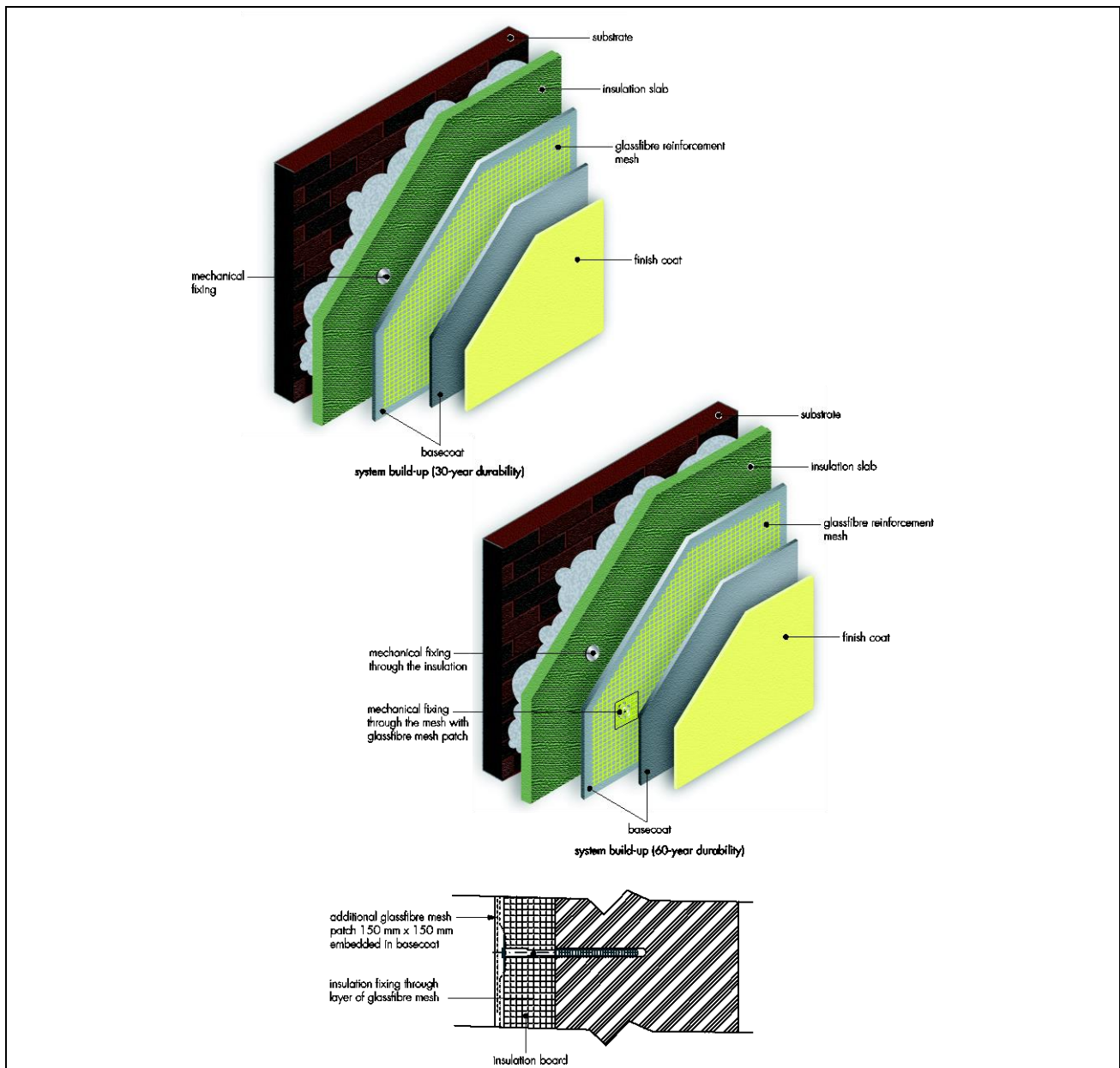
Figure 1 The K Systems M Silicone External Wall Insulation System
