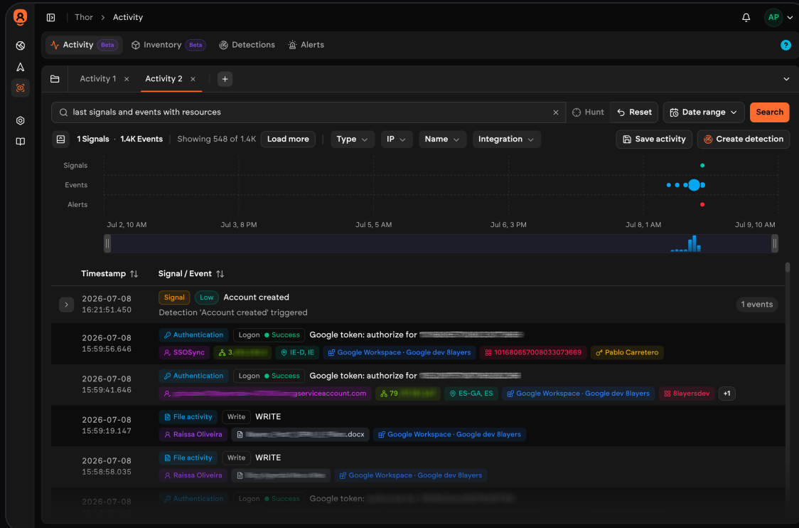
Activity workspace — threat hunting across signals and events
