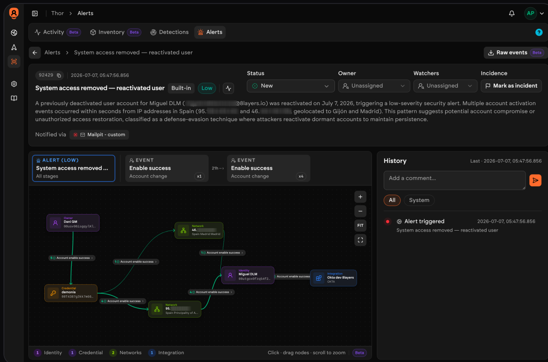
Alert detail with the identity graph reconstructing the attack path
