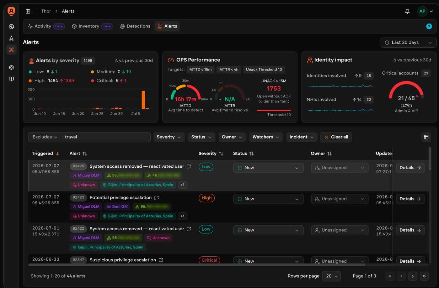
Thor — alert overview with severity trend and OPS performance (MTTD/MTTR)
