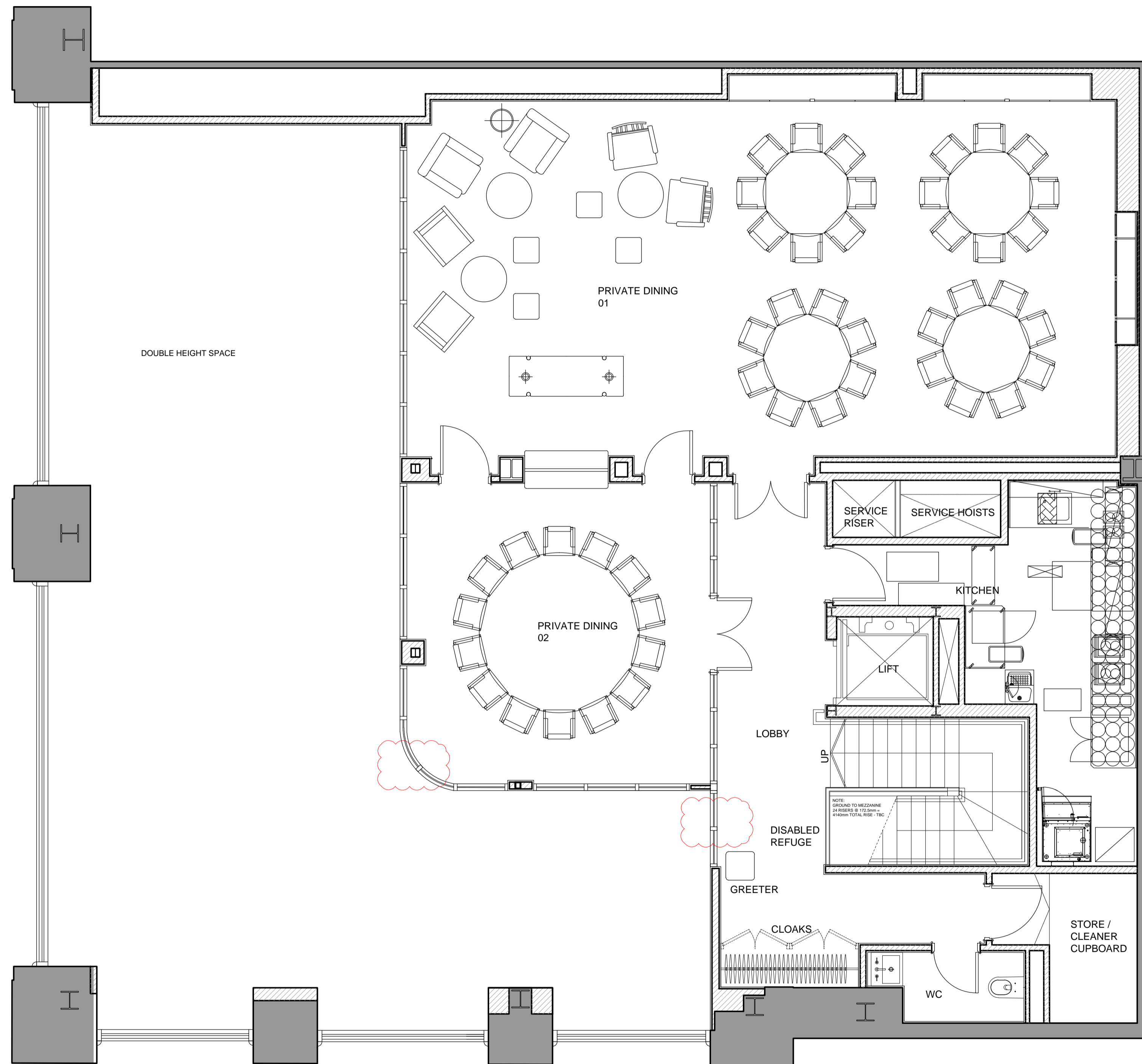
01 MEZZANINE GENERAL ARRANGEMENT PLAN SCALE 1:50
