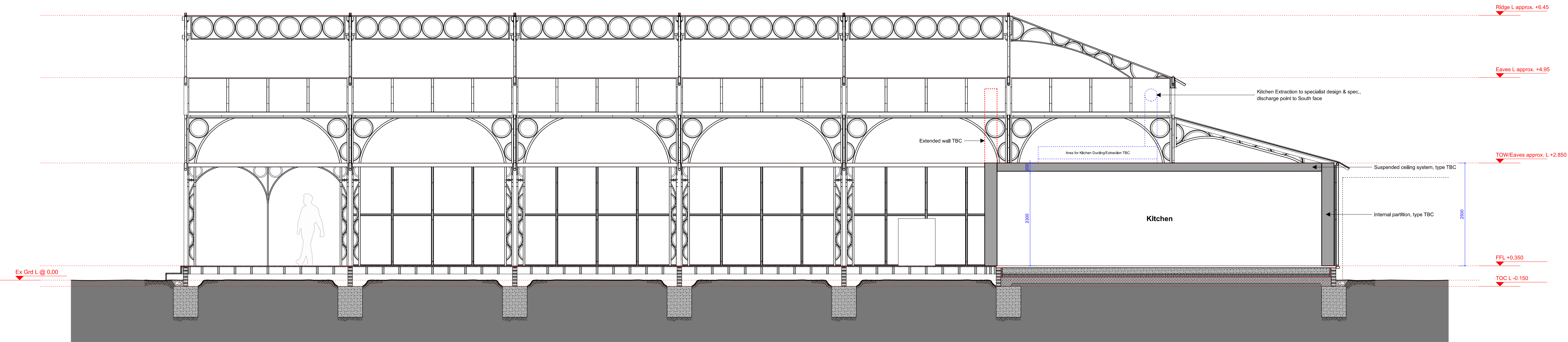
02 Section BB Scale 1:50 @ A1
