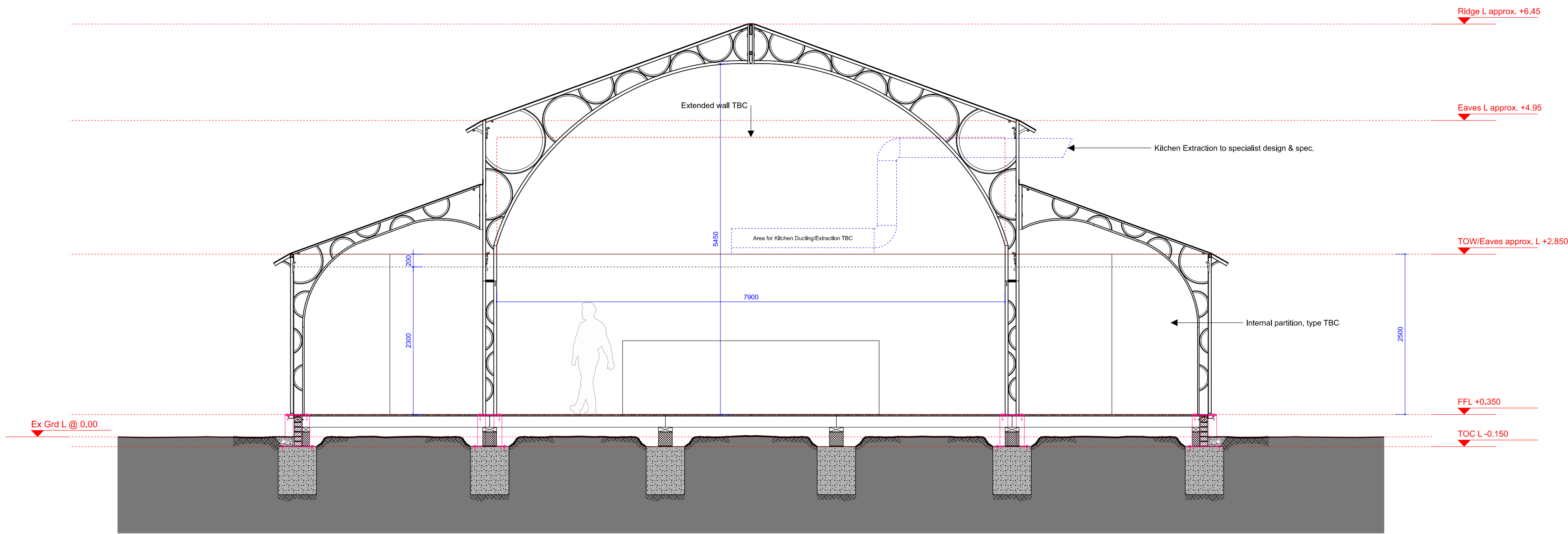
01 Section AA Scale 1:50 @ A1
