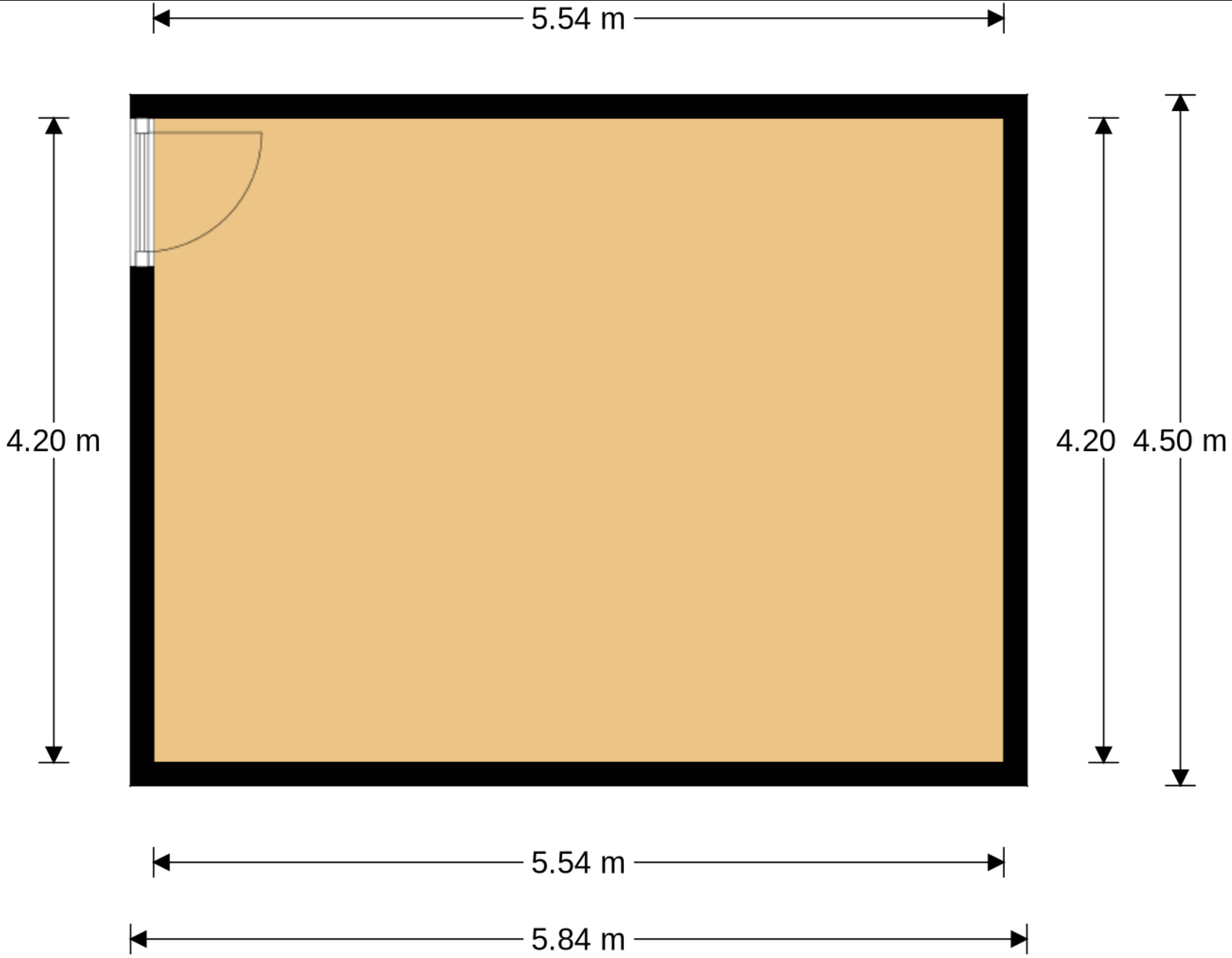
Ground floor
