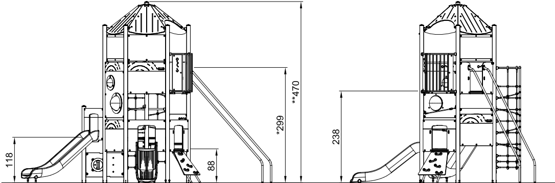
PCM111003 1:100
