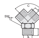
raccord taraudé
