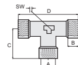
raccord taraudé
