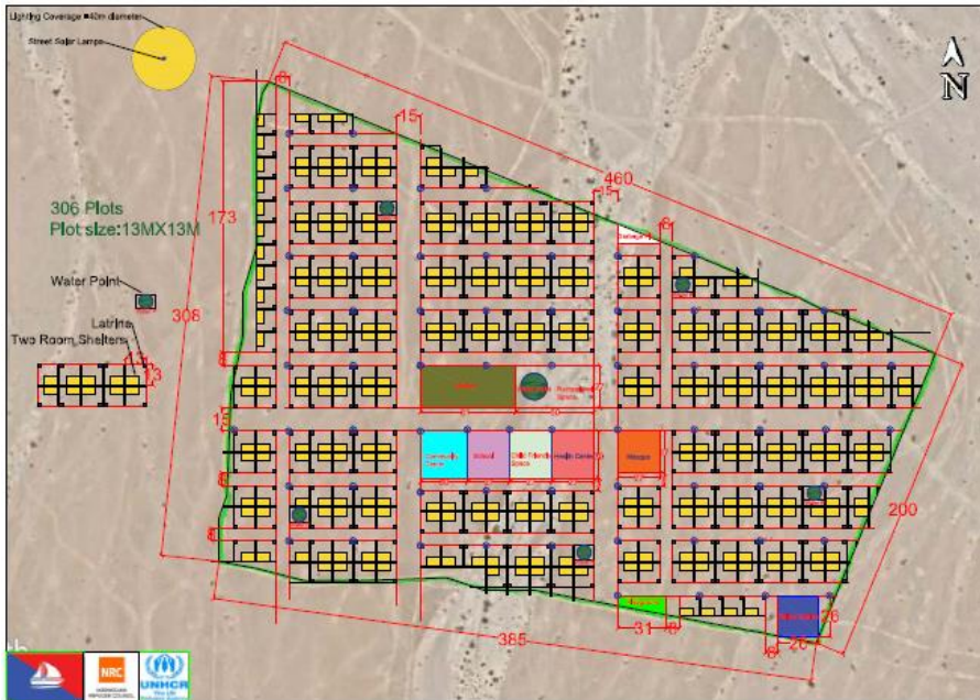
Site Plan for the relocation site in Girible settlement
