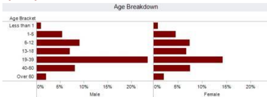
Figure 1: Age Breakdown
