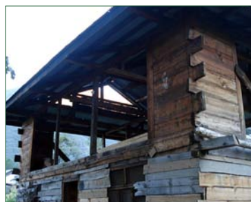
Thin boards may split or warp, nailed at weak location.
