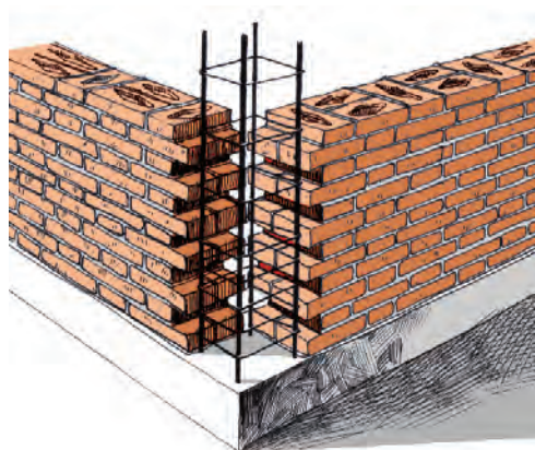
Patron flamand
