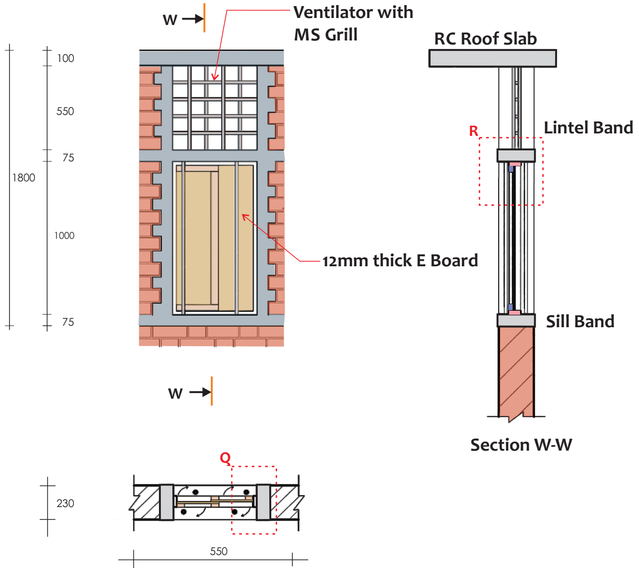
Window Details
