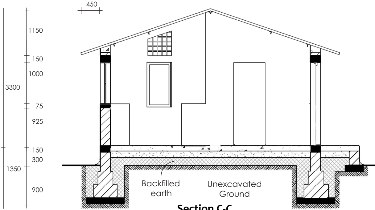
Section C-C
