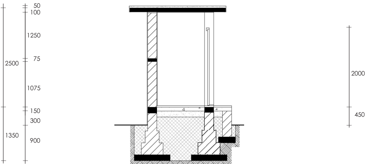
Section B-B
