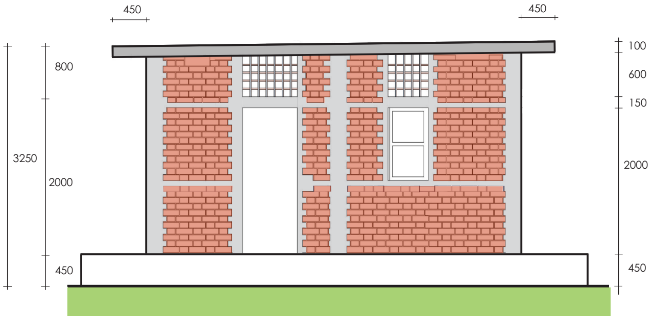
Left Elevation
