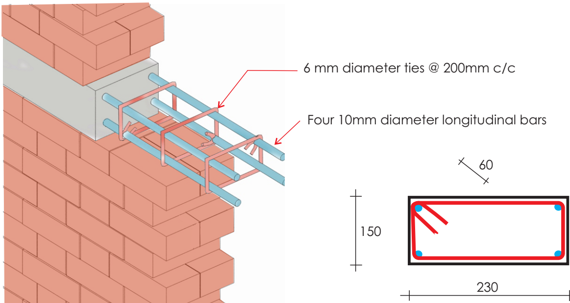
Plinth Band
