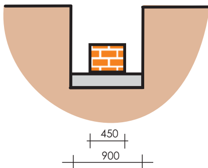
Brick Masonry
