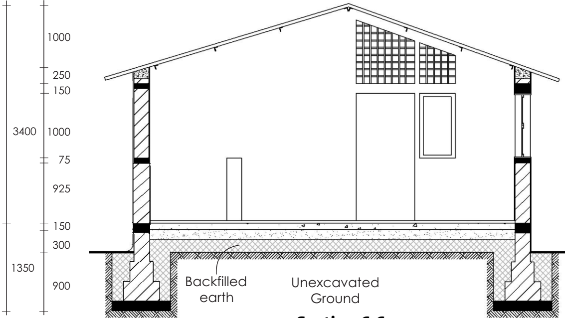
Section C-C
