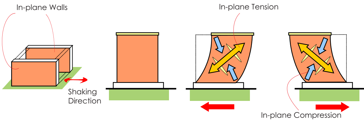
Shaking along length direction of masonry wall results in diagonal cracking
