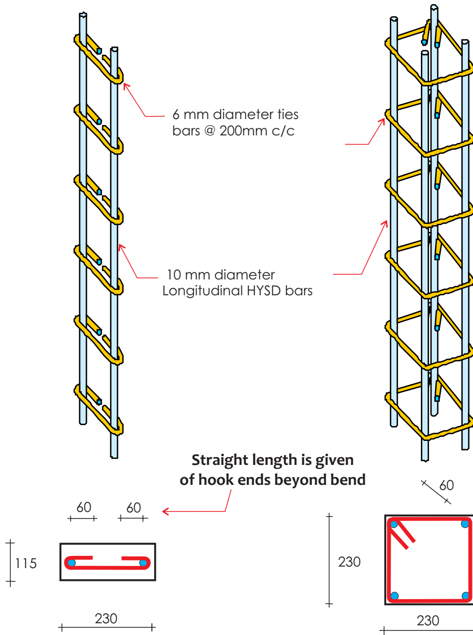
Reinforcement in Vertical RC confining members around door openings (230mm X 115mm)
