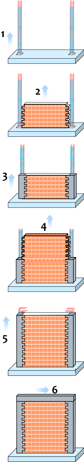
Sequence of Confined Masonry Construction
