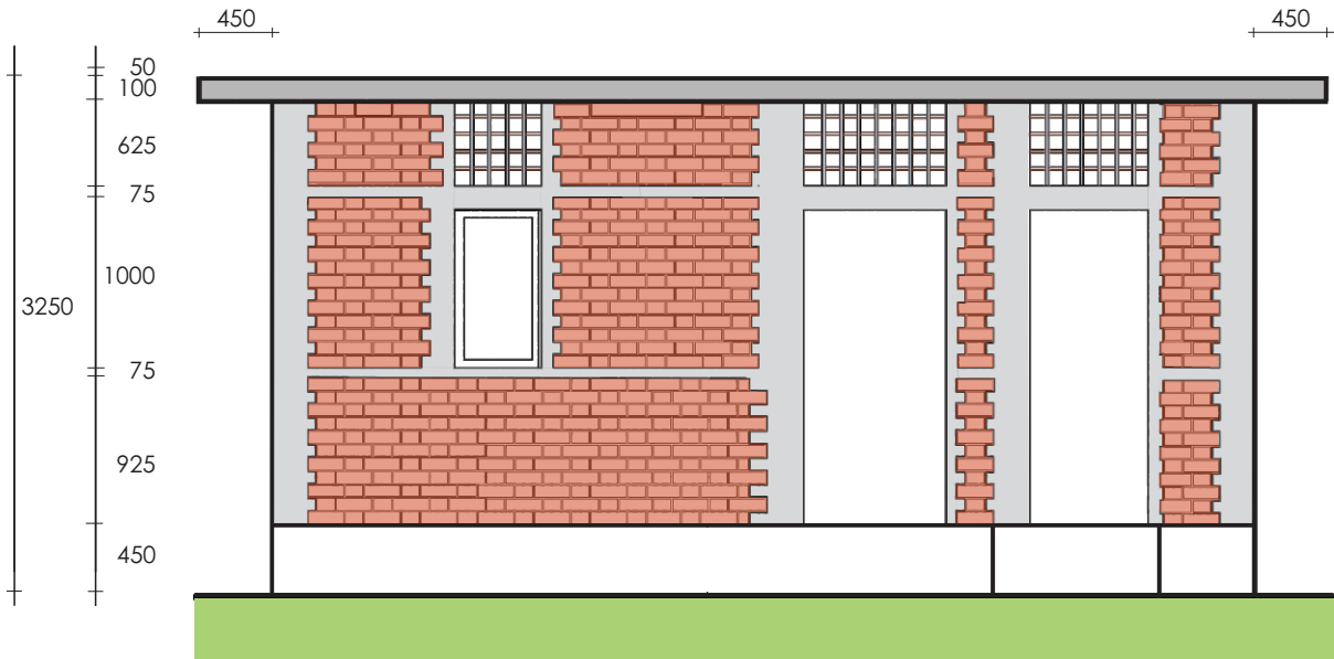
Back Elevation
