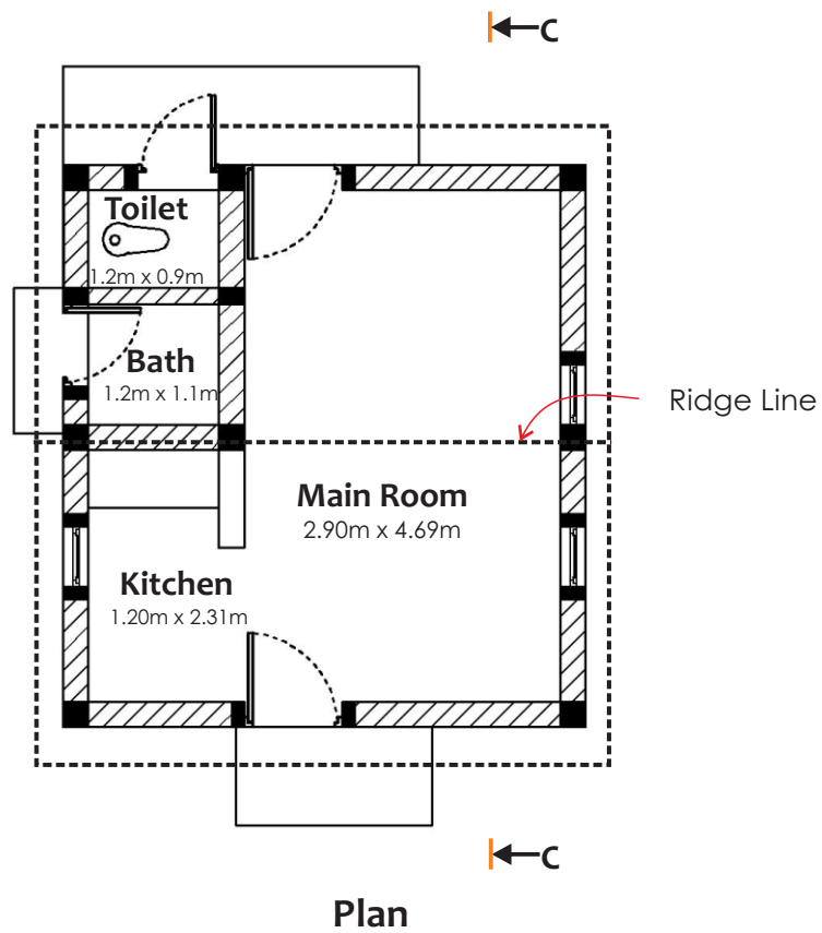
House with sloping roof
