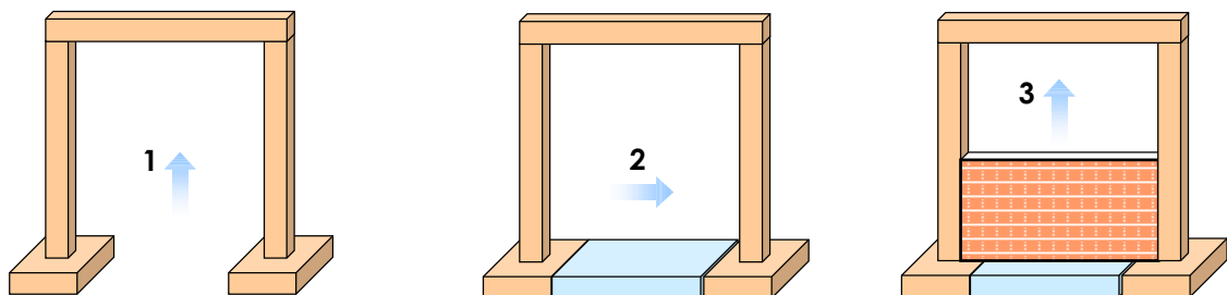
Sequence of RC frame construction with URM infill walls
