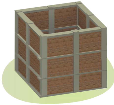
Masonry wall segments confined on all sides with RC elements
