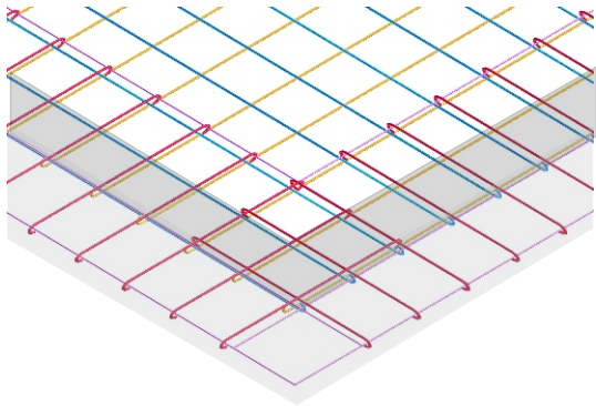
Reinforcement at Slab Corner Edge
