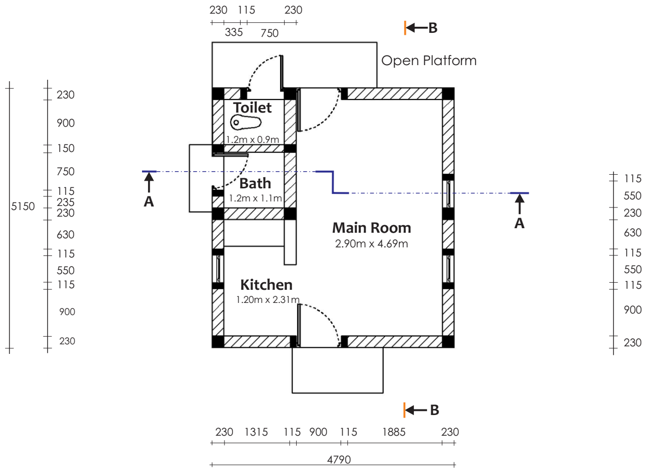
Plan
