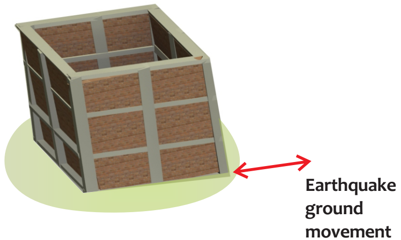
RC elements prevent masonry from collapsing
