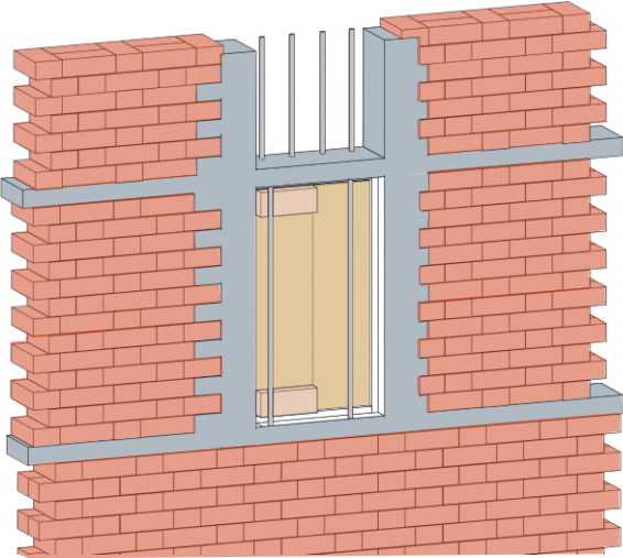
Pivoted Window Closed Position
