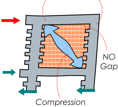
Only nominal bending in RC vertical and horizontal elements
