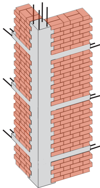
Vertical RC elements keep brick masonry segments in place at the corners
