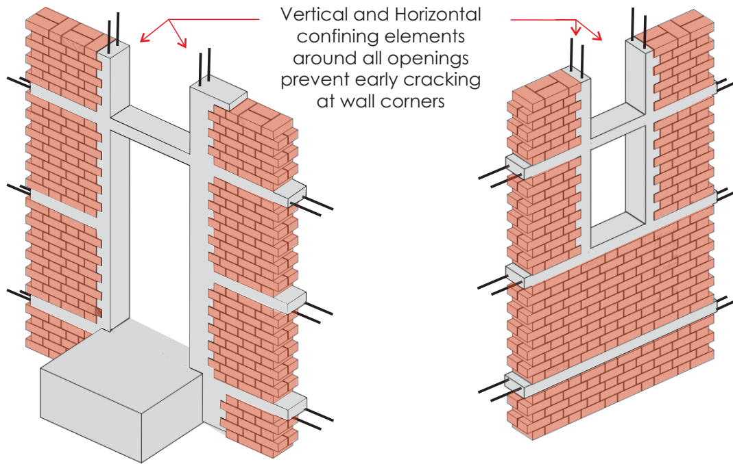
Lintel, Sill and Plinth bands pass through the vertical RC elements RC bands and elements support the brick masonry at openings
