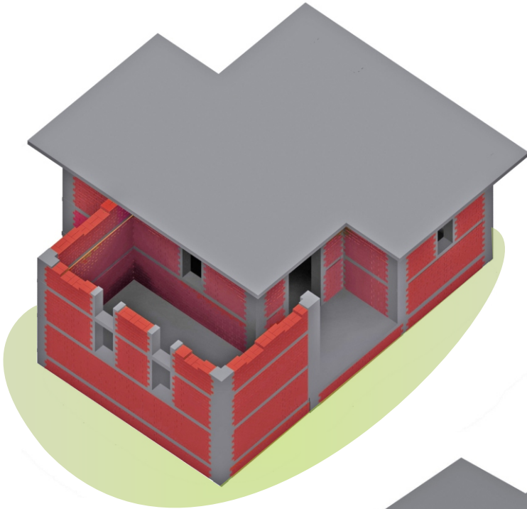
Option 3 Extended Built-up area: 47.94 m 2 Carpet area: 32.20 m 2
