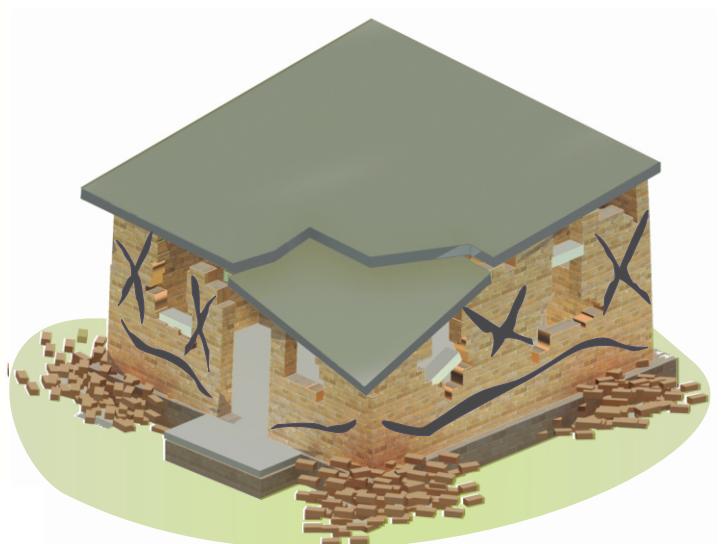
Severe Shaking Walls collapse and slab falls
