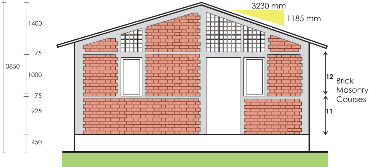
Front Elevation
