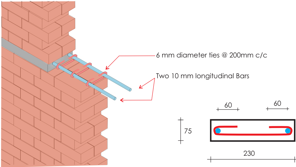
Sill and Lintel Bands
