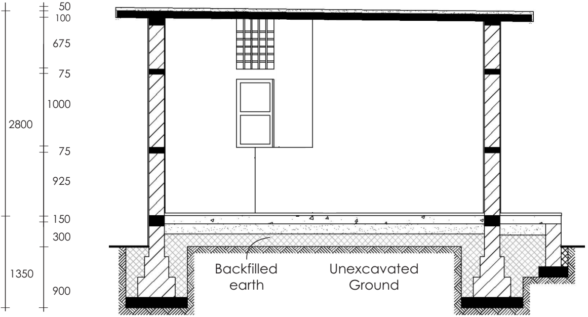
Section B-B
