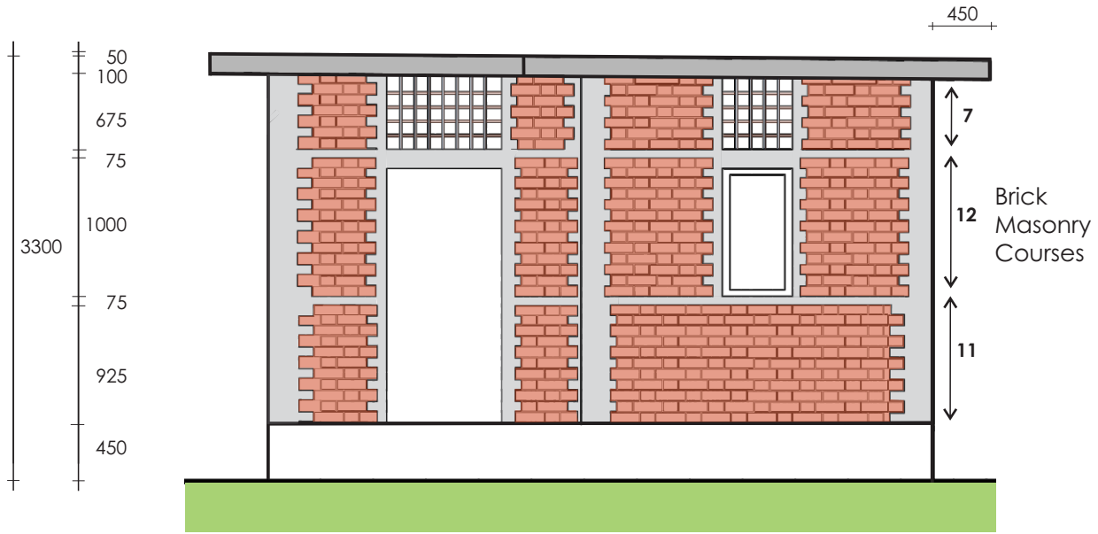
Front Elevation
