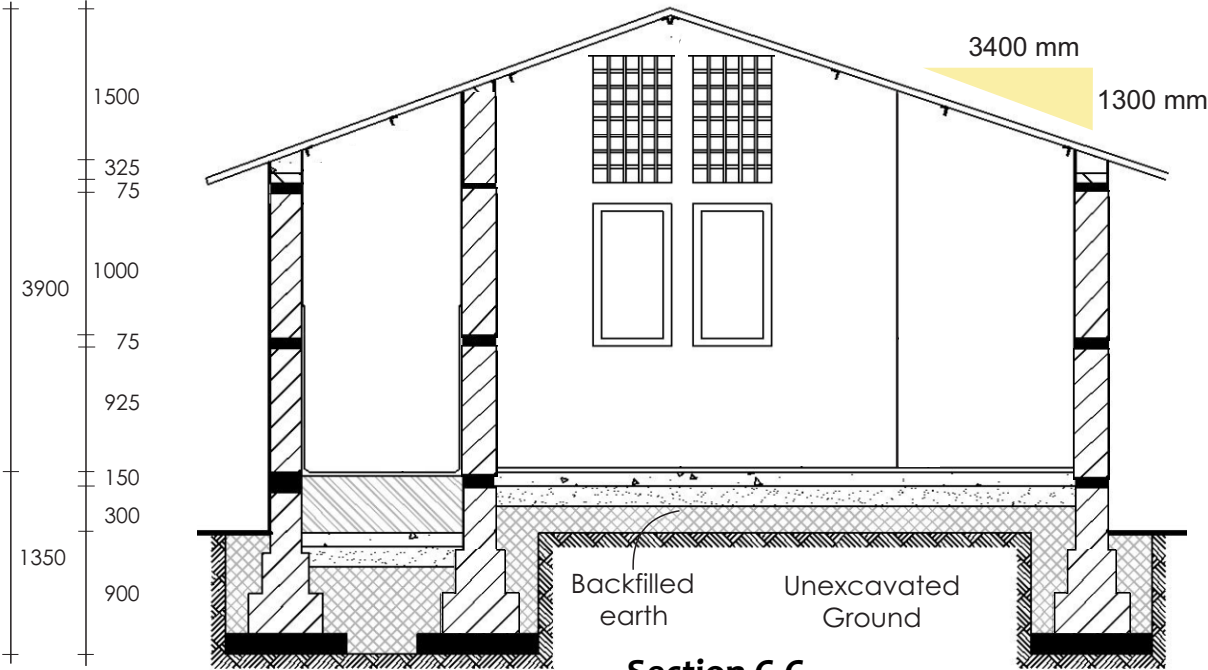
Section C-C
