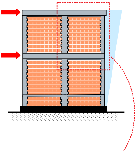
Only nominal bending in RC vertical and horizontal elements
