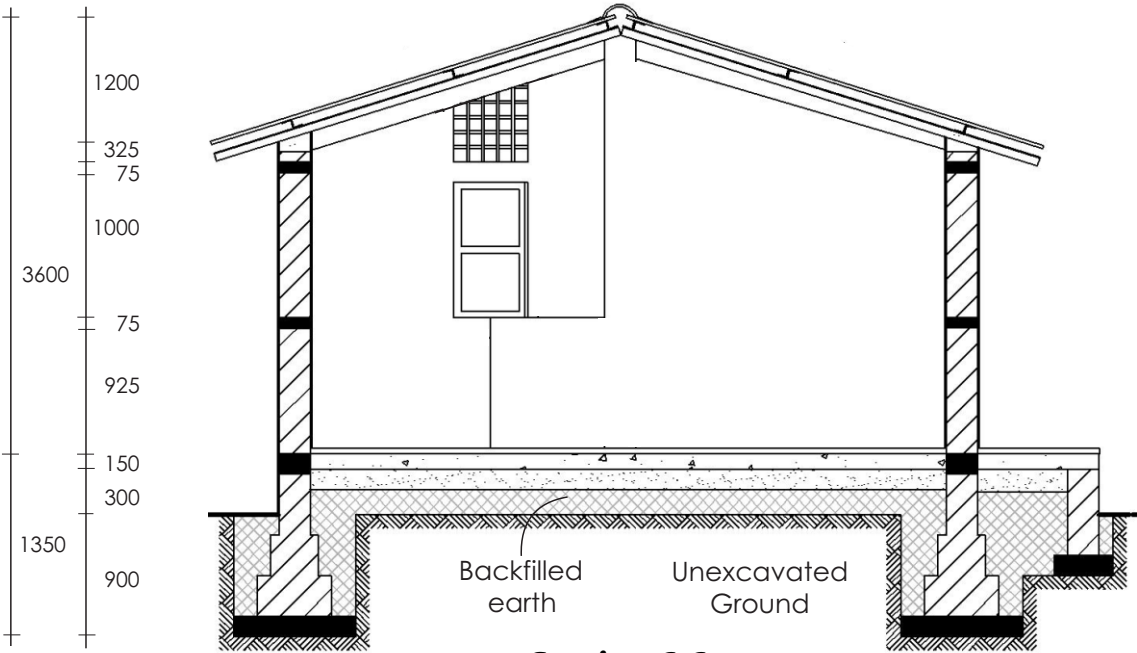
Section C-C
