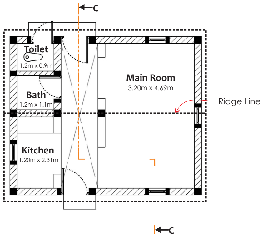
Plan
