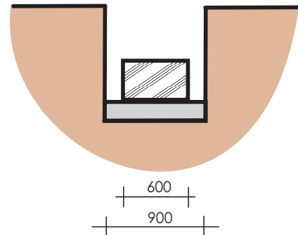
Stone Masonry
