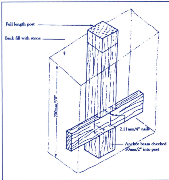
Wooden post with anchor beam
