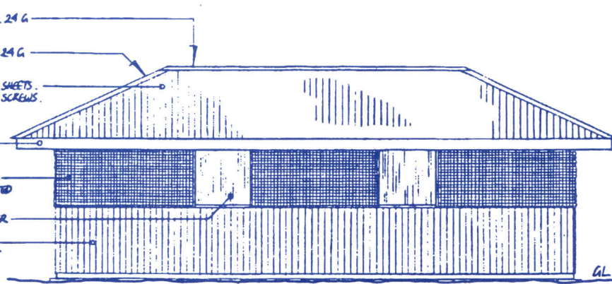
FINISHED ELEVATION 1
