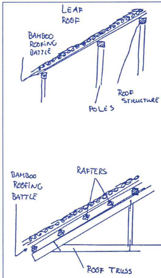
Construction principles for leaf roofs
