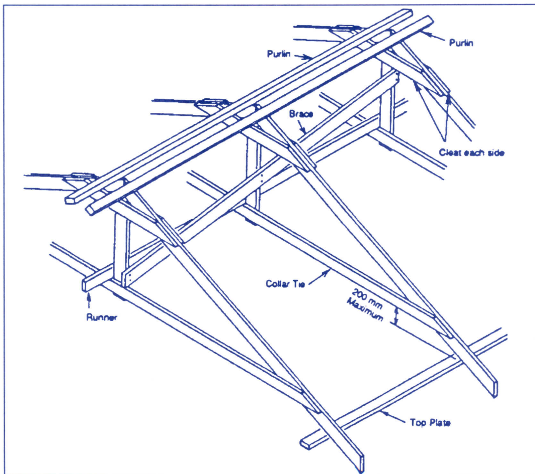
Bracing together the roof trusses
