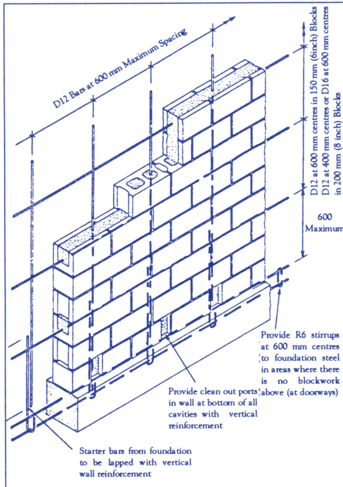
Typical concrete block wall details
