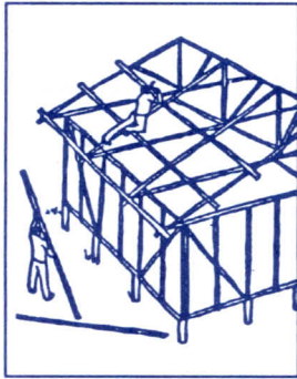
Nail purlins in place
