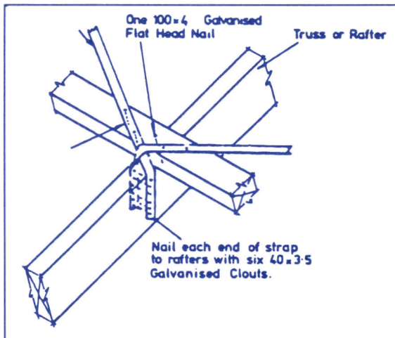
Detail for fixing roof straps
