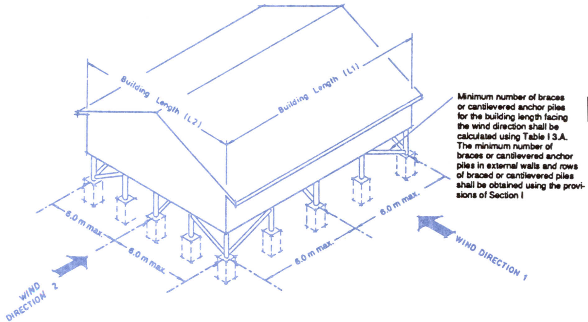
Bracing schedule for a wooden frame house
