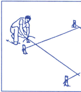
Use string to lay out the house
