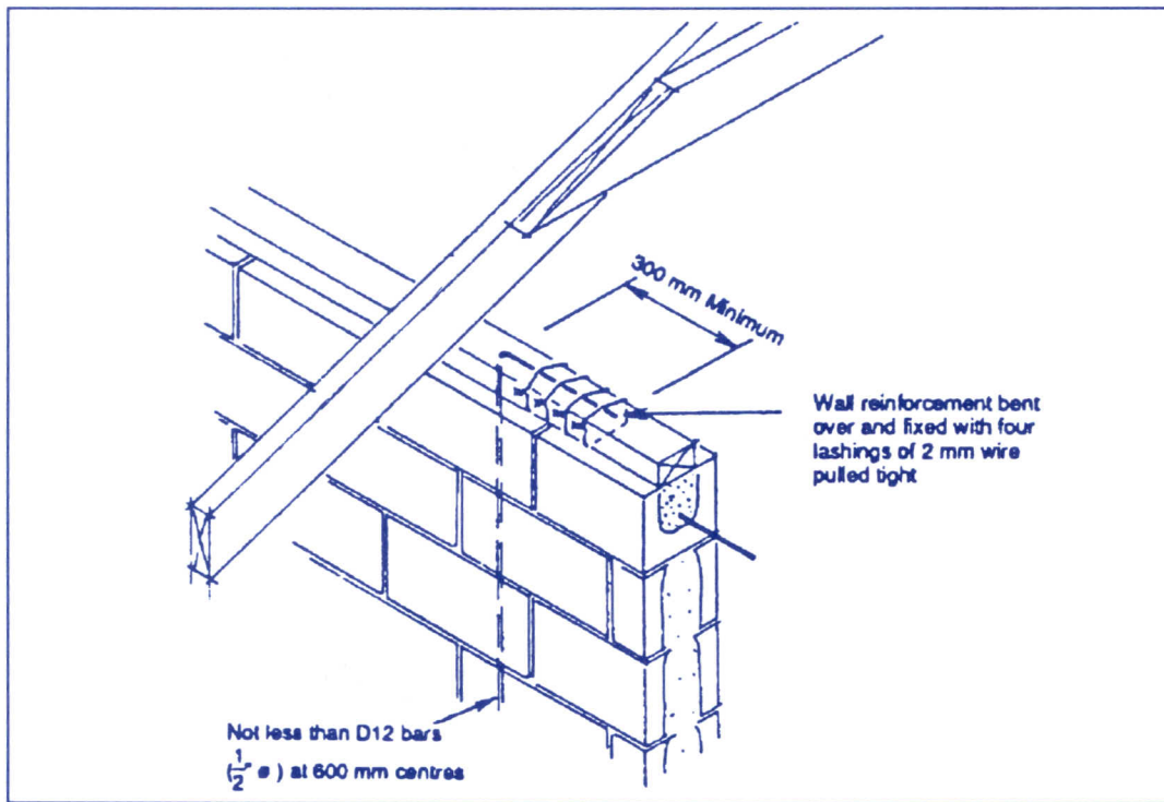
Fixing the top plate using vertical reinforcement bars
