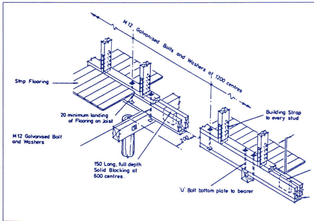
Wall to floor connection details
