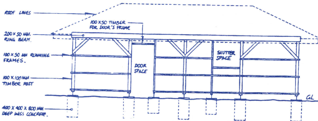
FRAMES ELEVATION 3
