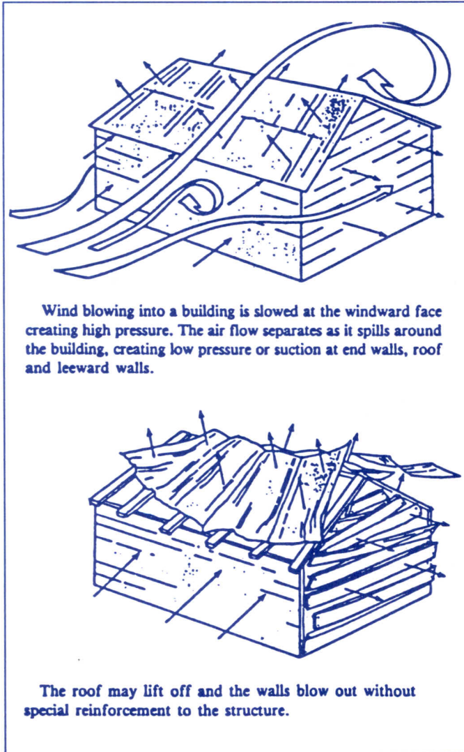
How a cyclone damages a building
