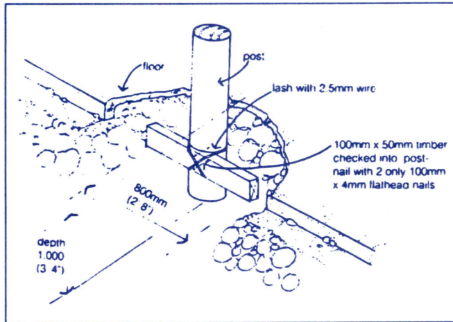
Detail of a post base using wire lashes
