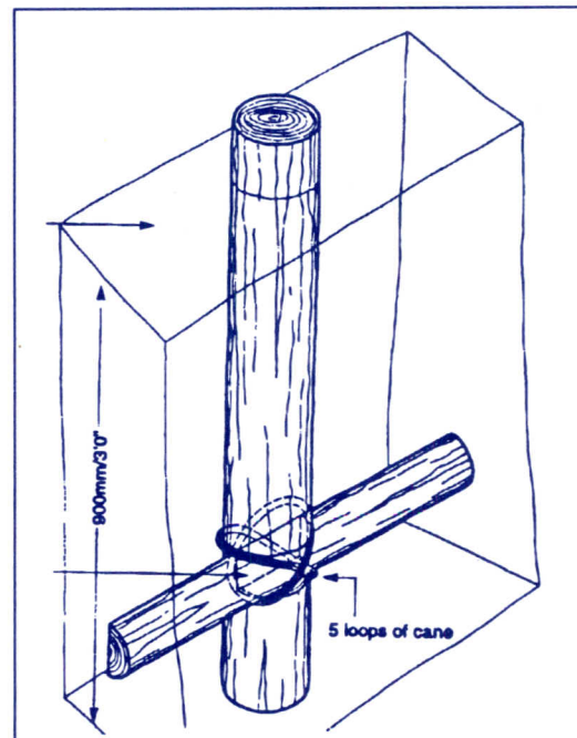
Anchoring posts with an anchor beam
