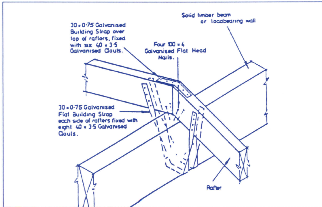
Strapping the rafter to the roof beam
