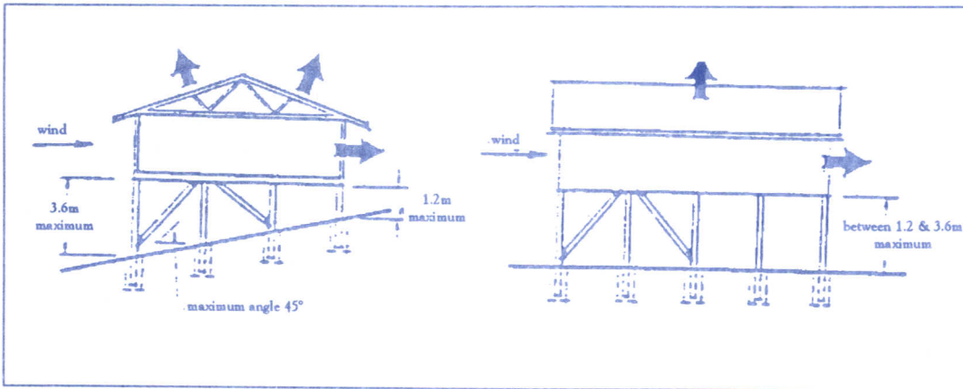
Bracing of piles to resist wind forces
