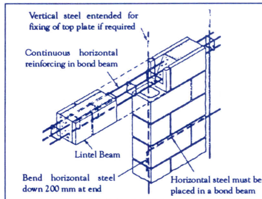
Fixing horizontal ring beam to vertical reinforcement
