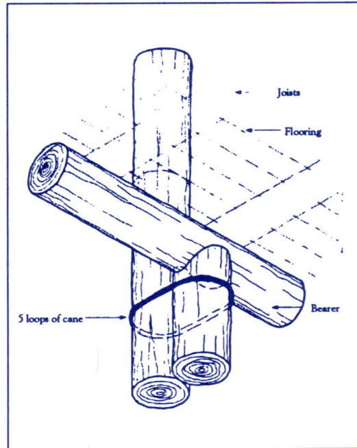
Tie post and floor bearer together for sufficient strength
