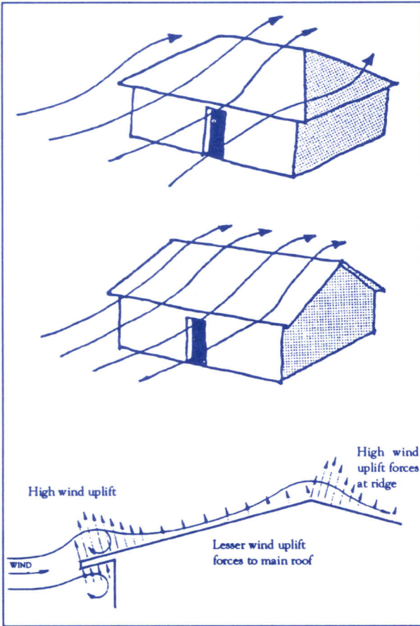
Wind flow and forces on the roof
