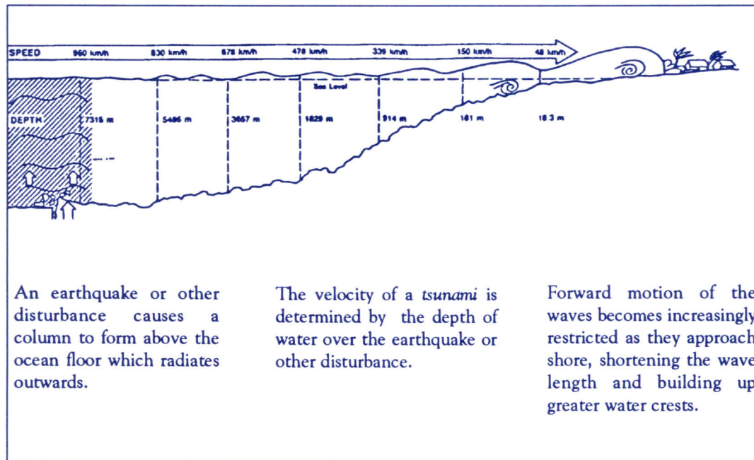
Development of a tsunami
