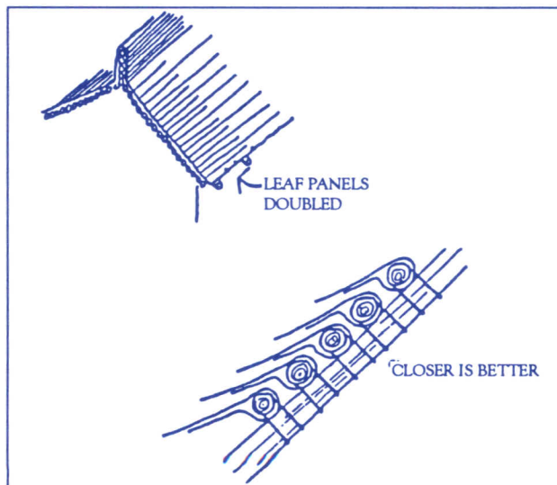
Principles for fixing leaf roof covers
