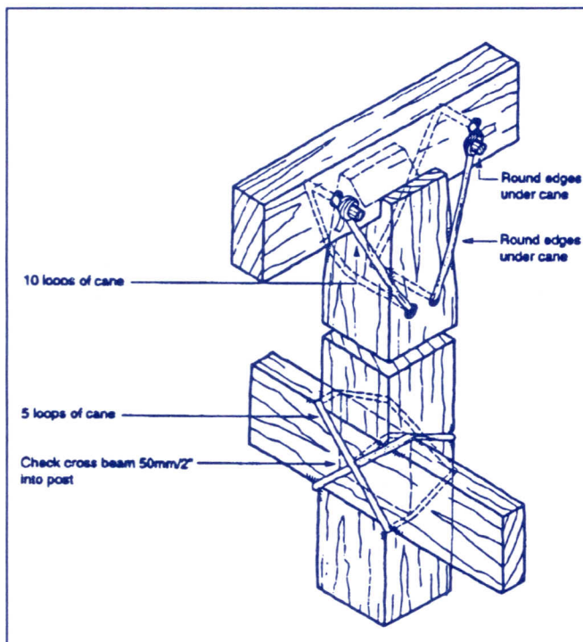
Post to floor connection using traditional straps
