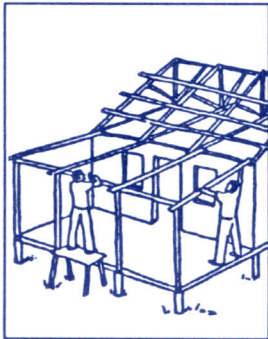
Set rafters at veranda
