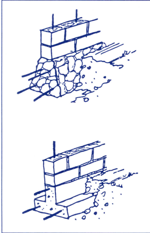
Two types of reinforced foundations: T-slab and concrete with rocks
