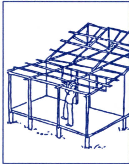
Nail purlins to rafters
