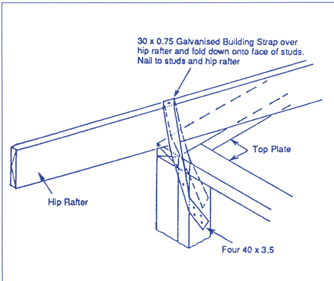
Strapping the rafter to wall post and top plate
