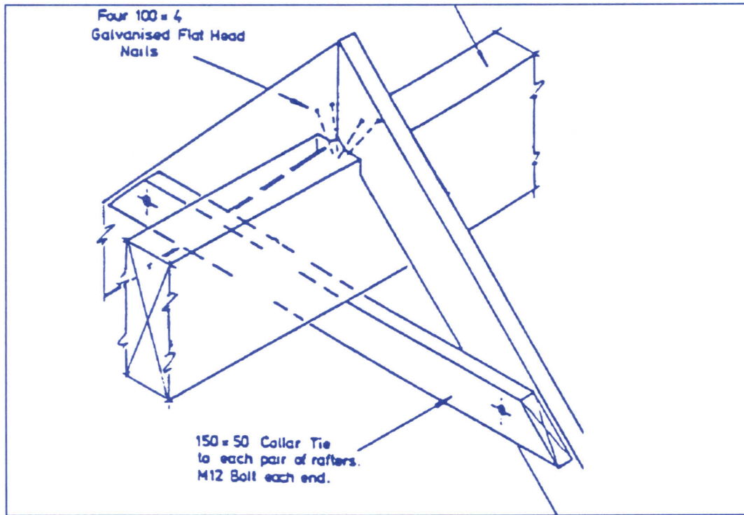
Alternative using a collar tie to fix rafters
