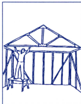
Put truss on wall
