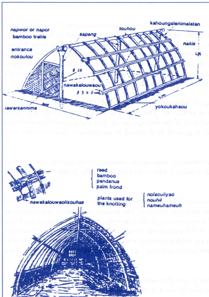
View of a frame and interior of a cyclone shelter in Tanna, Vanuatu
