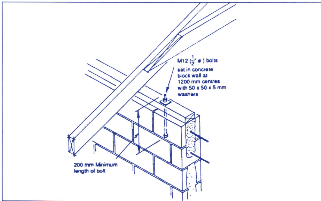
Fixing the top plate with M12 bolts
