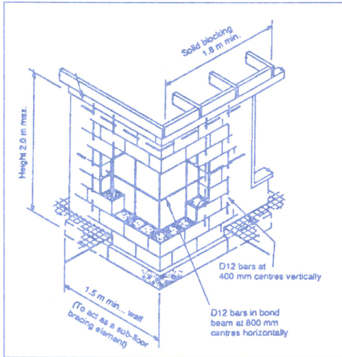
Details of a concrete block corner foundation wall
