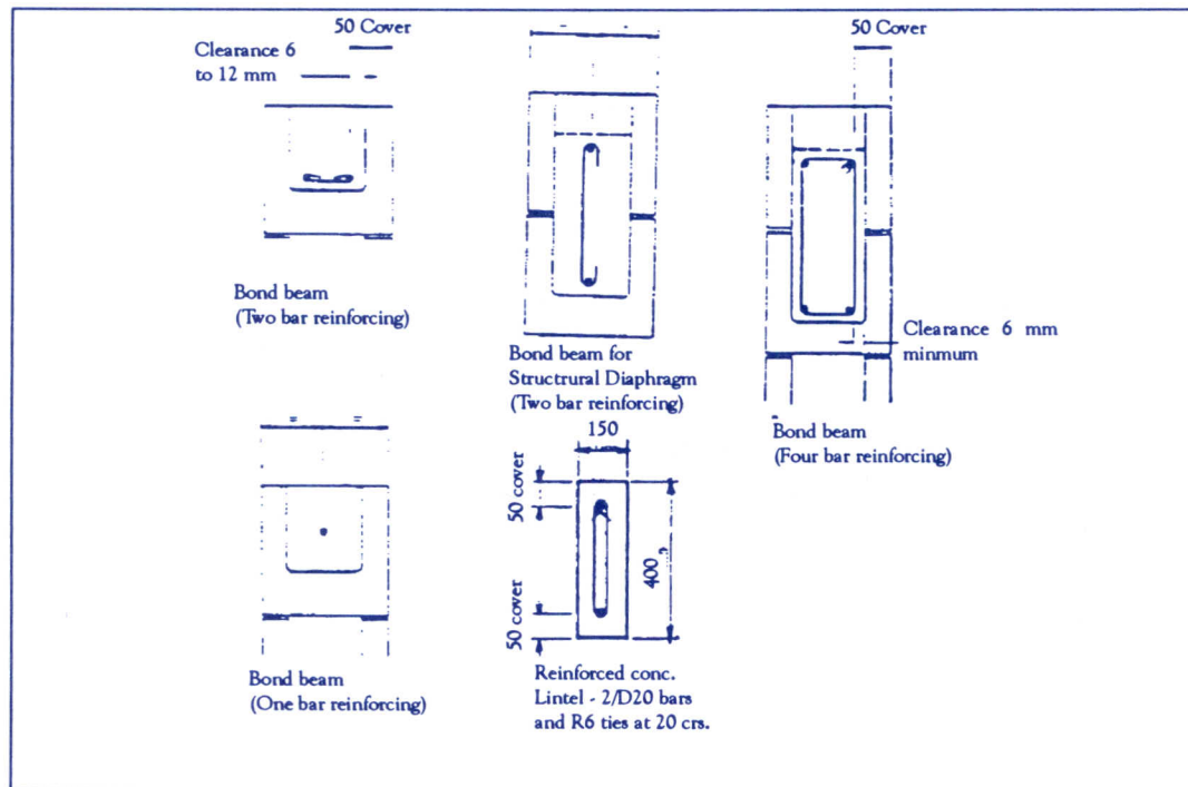
Details of concrete ring beam with reinforcement
