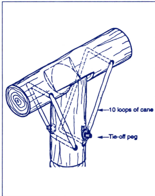
Details for connecting wooden poles with cane
