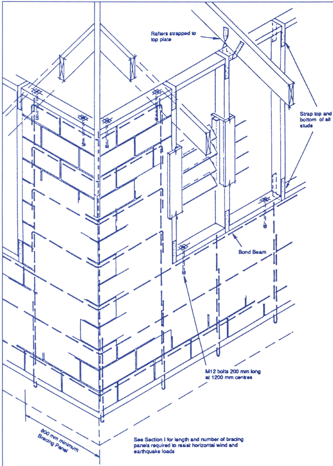
Detail of a concrete block bracing wall
