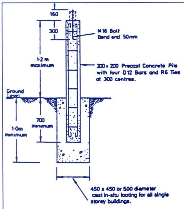
Detail of a pre-cast concrete pile
