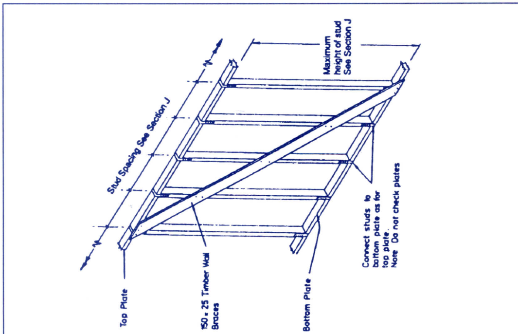
Connection of braces to the wall
