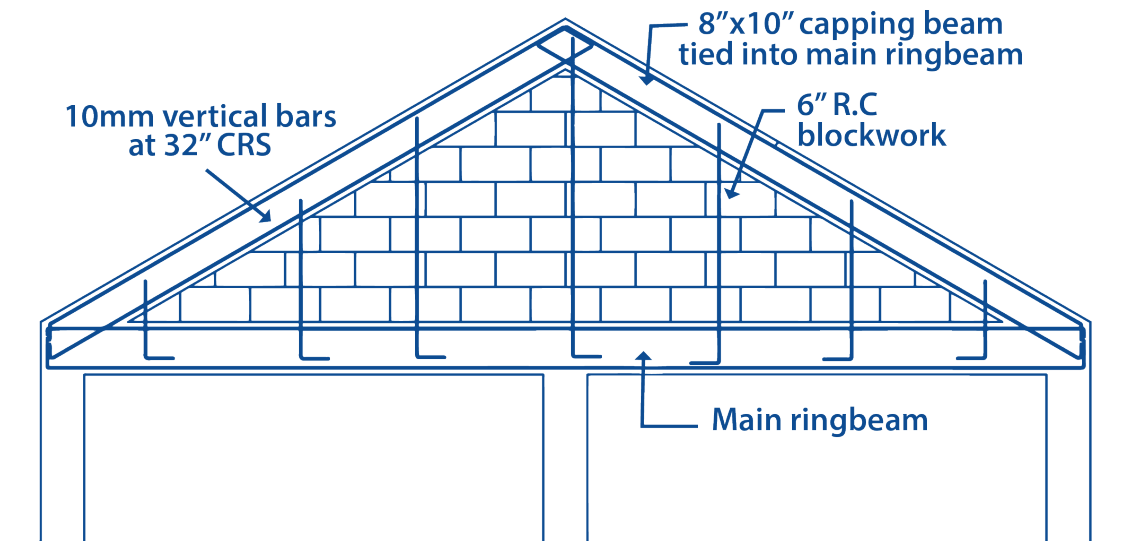
GABLE END DETAIL
