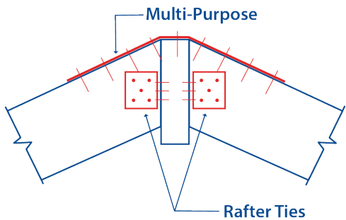
RAFTER/ RIDGE ELEVATION
