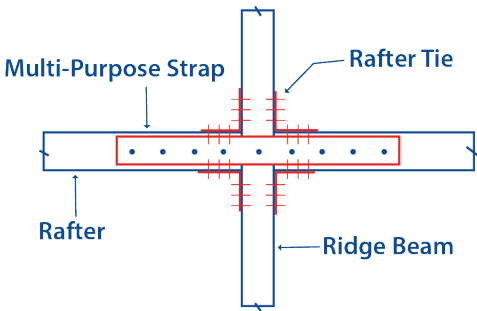
RAFTER/ RIDGE PLAN
