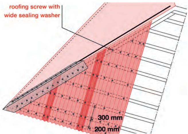
Position of fasteners on a 15° hipped roof with wind speed &lt; 250 km / h
