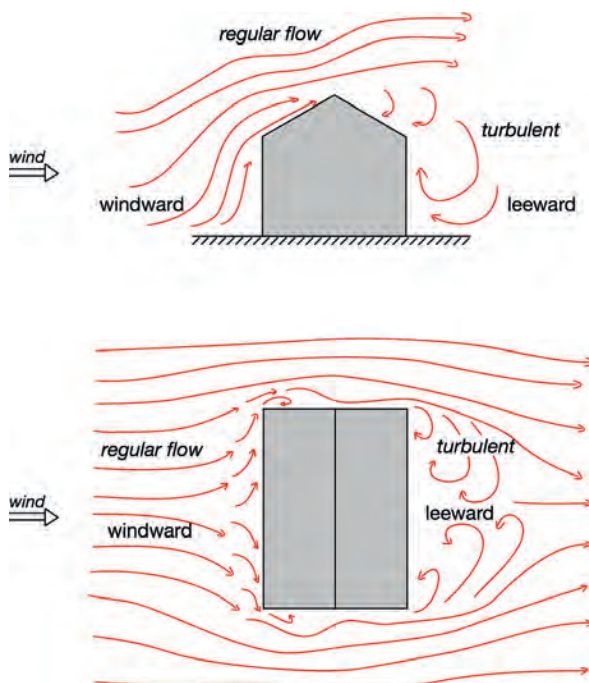
Wind flow on a rectangular building
