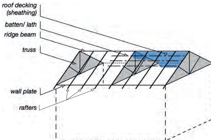
Drawing 3 – terminology of the structure of gable roofs
