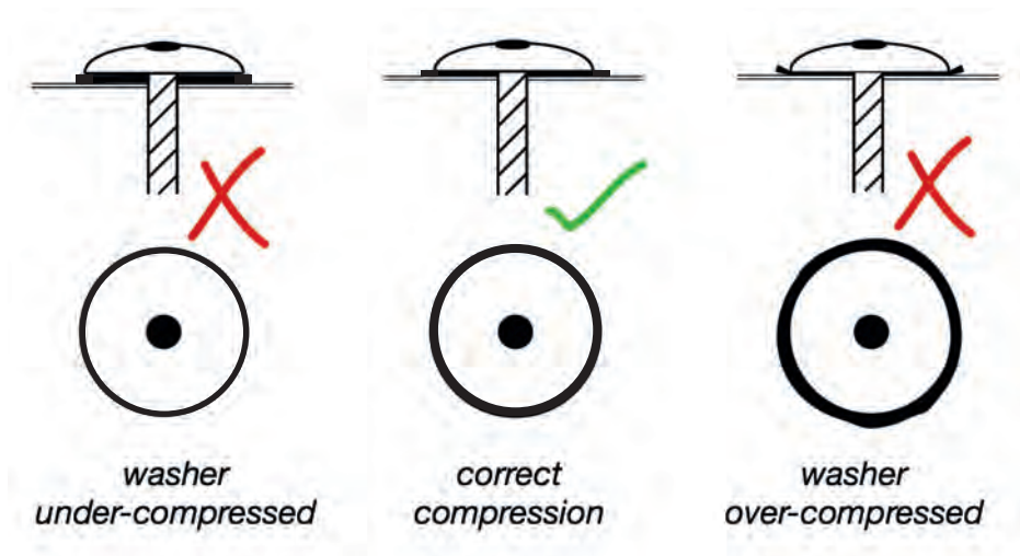
Compression of rubber washer
