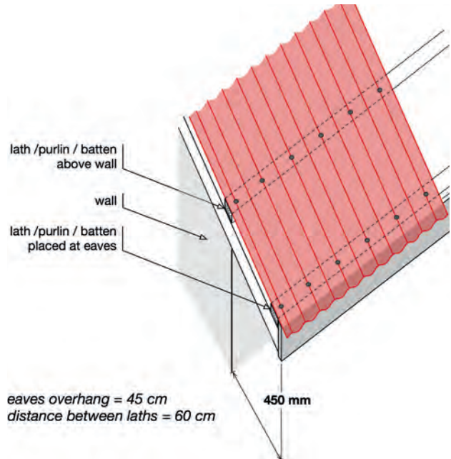
Location of laths / battens at eaves overhang (case of short eaves)
