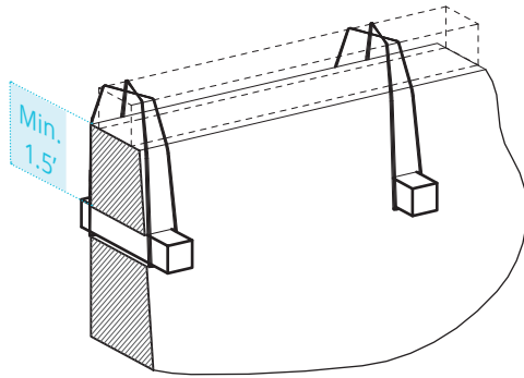
A Tie Connection A wooden peg is cast into the wall and wire used to secure the ring beam. This option is easier to build and appropriate for timber and bamboo ring beams.
