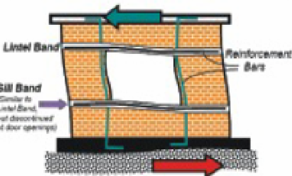
No cracks in building with vertical reinforcement
