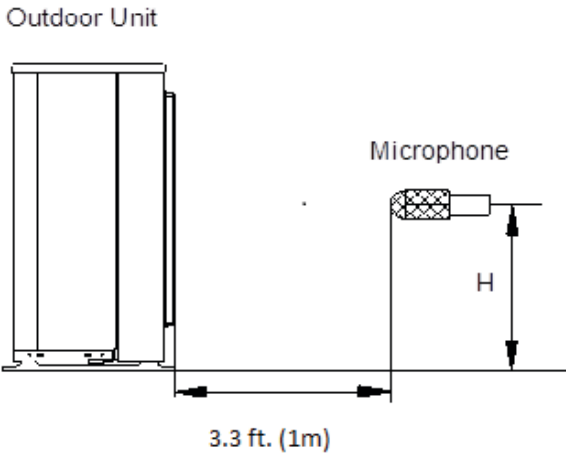
Fig. 7 – Outdoor Unit Sound Pressure Test Conditions NOTE: H=0.5 x Height of outdoor unit
