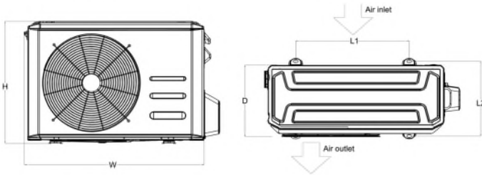
OUTDOOR UNIT DIMENSIONS
