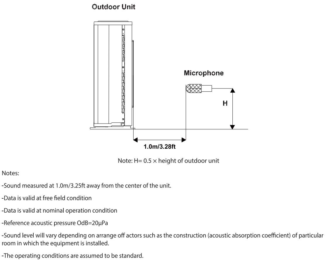
Fig. 17 —Sound Pressure Testing Method
