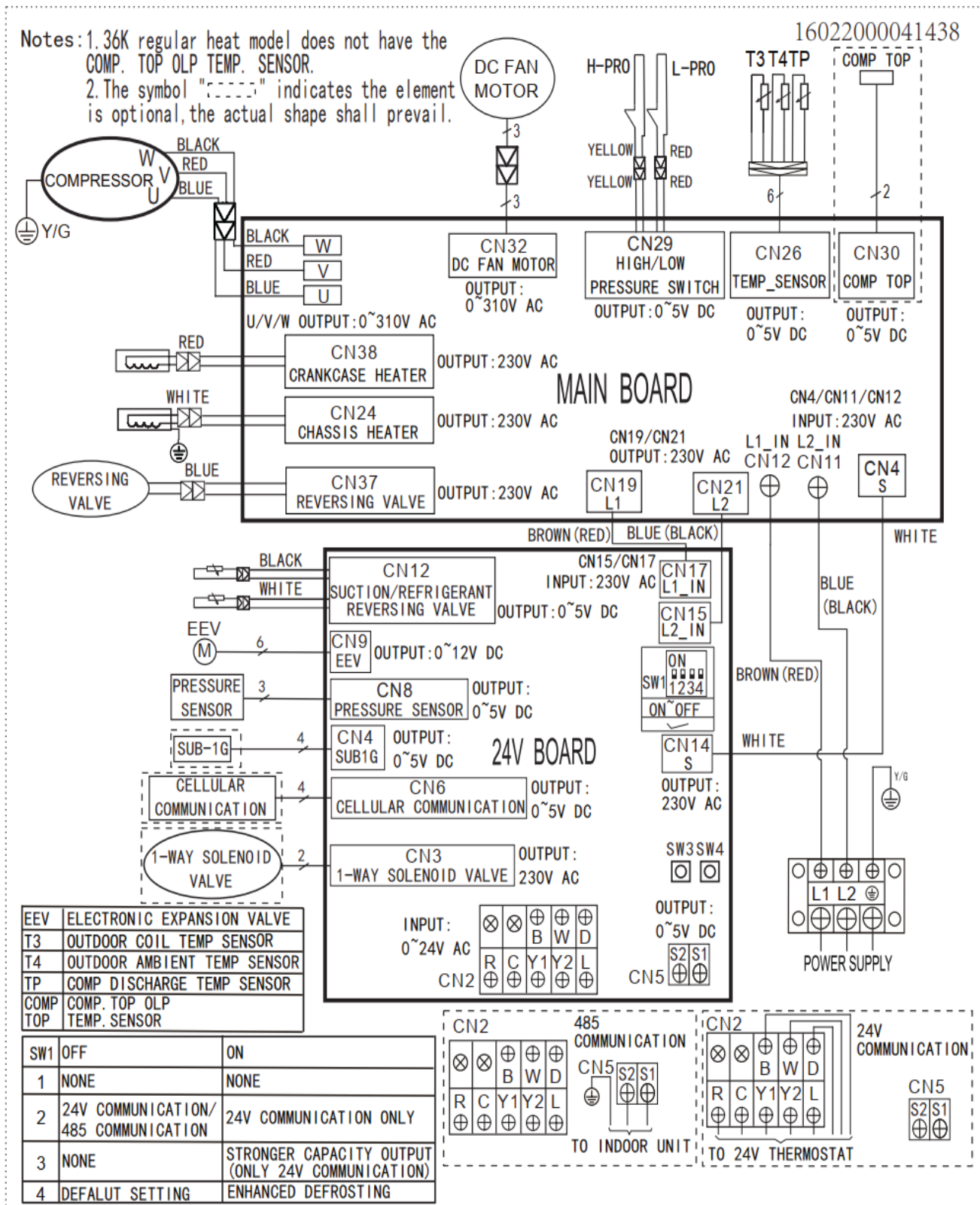
Fig. 38 — Wiring Diagram Size 30K
