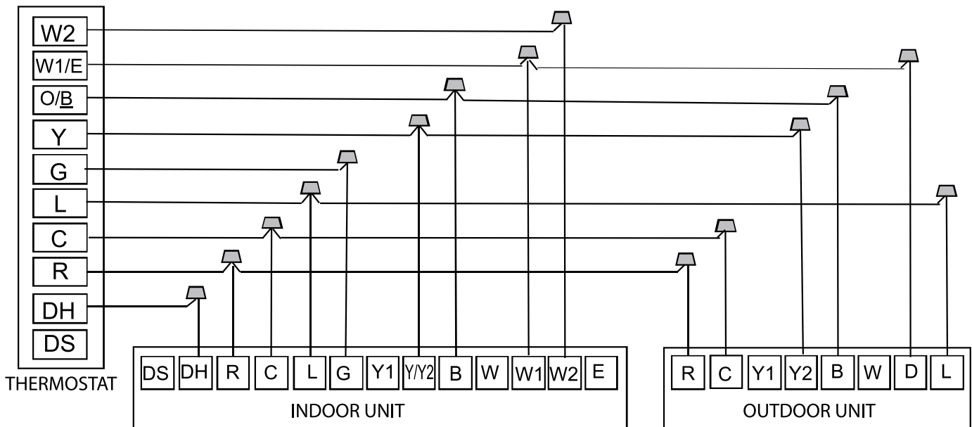
Fig. 29 —Wiring for 4H and 2C thermostat
