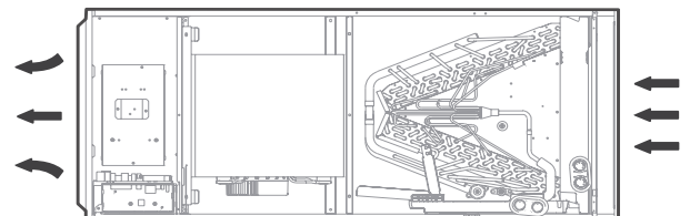
Fig. 10 – Horizontal Left installation
