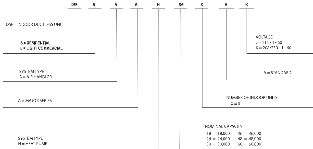
Fig. 6 – Model Number Nomenclature
