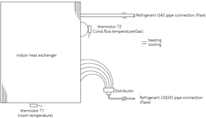
Fig. 26 – Refrigerant Systems Diagram
