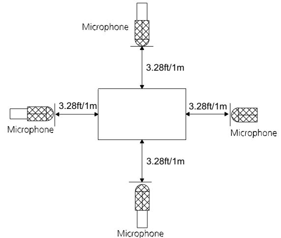
Fig. 18 —Vertical Installation
