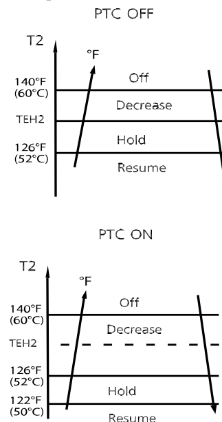
Fig. 5 – Evaporator Coil Temperature Protection
