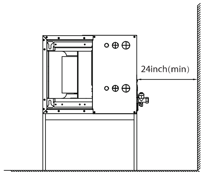
Fig. 13 – Horizontal Installations
