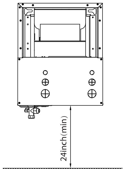
Fig. 12 – Vertical Installations
