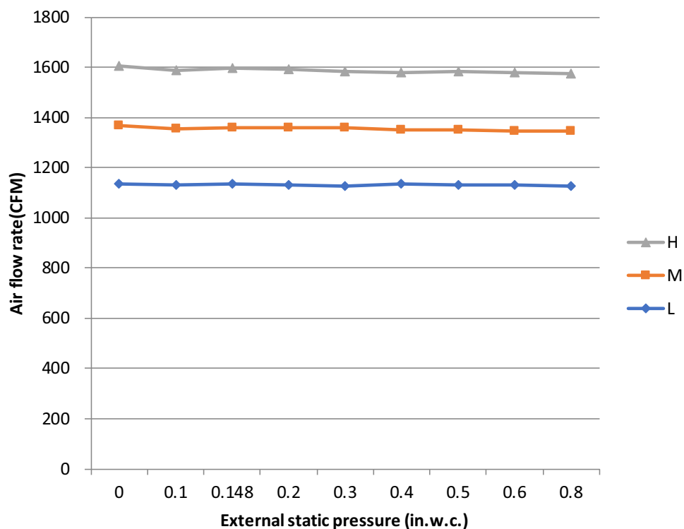
Fig. 34 — 60k (Vertical, Horizontal Right, Horizontal Left)
