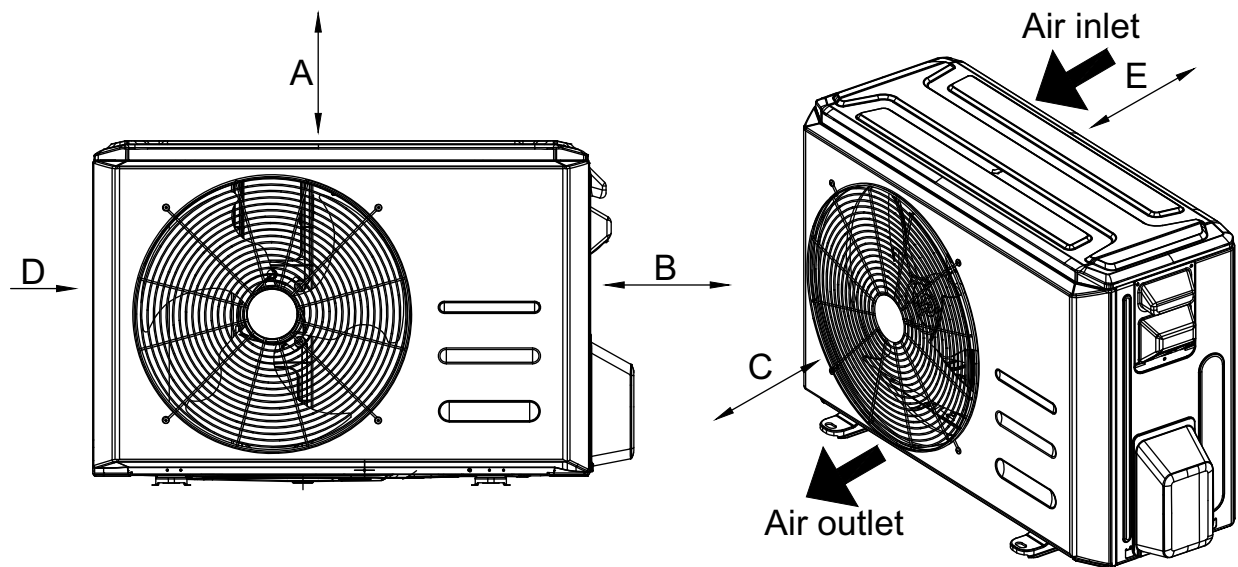
Fig. 6 — Clearances
