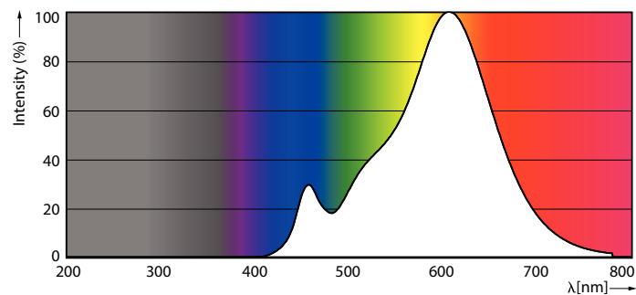
Spectral Power Distribution Colour - MAS LED Sensor ND 8-60W A60 E27 827
