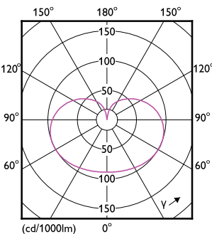
Light Distribution Diagram - MAS LED Sensor ND 8-60W A60 E27 827
