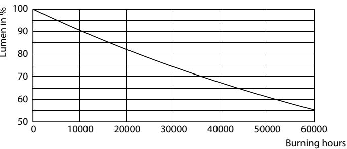
Lumen Maintenance Diagram - RS060B LED5-36/827 PSR II WH LILO
