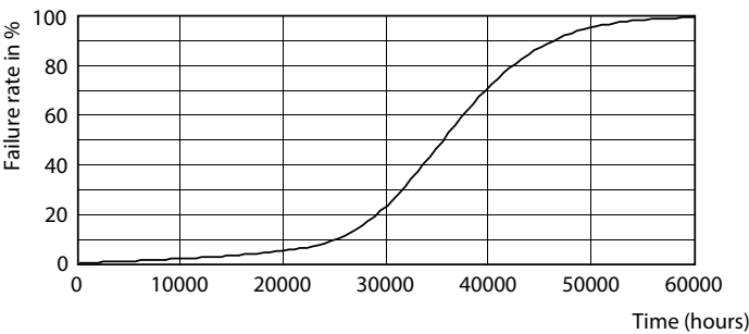
Life Expectancy Diagram - RS060B LED5-36/827 PSR II WH LILO
