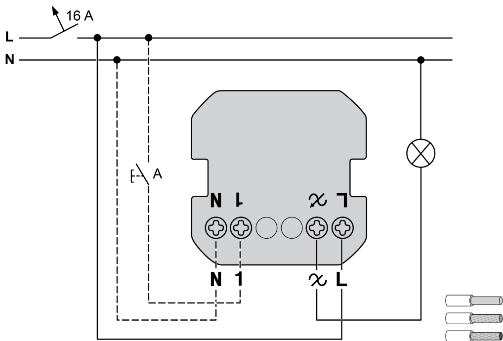
A - Mechanical push-button (optional)
