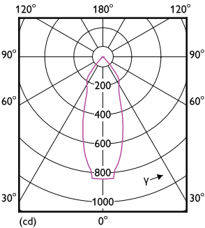
Light Distribution Diagram - RS061B LED5-36/830 PSR II WH LILO
