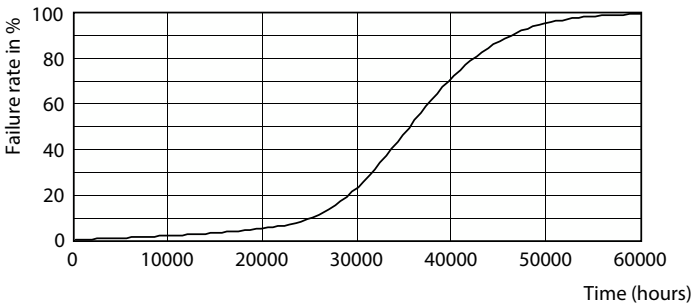
Life Expectancy Diagram - RS061B LED5-36/830 PSR II WH LILO
