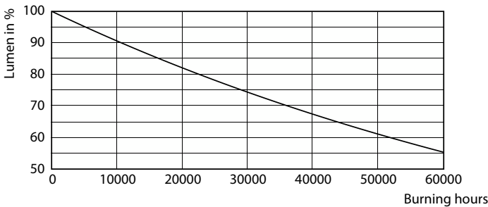
Lumen Maintenance Diagram - RS061B LED5-36/830 PSR II WH LILO
